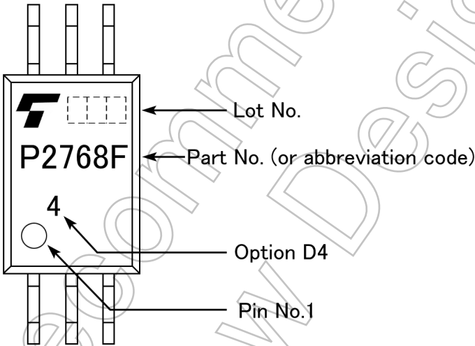
Fig. 16.3 Marking Example (Note)
