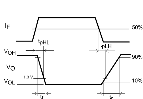
Fig. 12.1.7 Switching Time Test Circuit and Waveform
