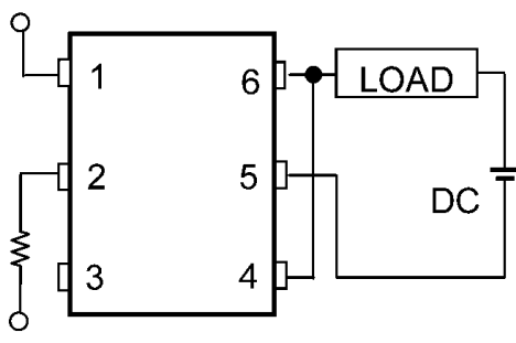
Fig. 12.2.3 C Connection
