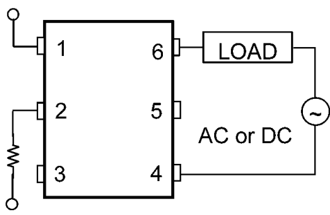
Fig. 12.2.1 A Connection
