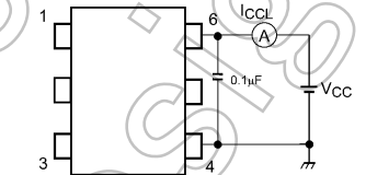
Fig. 12.1.6 I_{CCL} Test Circuit
