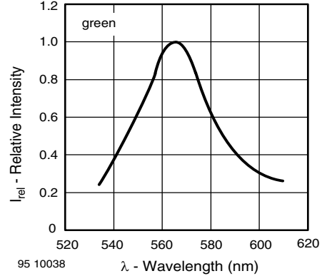
Fig. 18 - Relative Intensity vs. Wavelength
