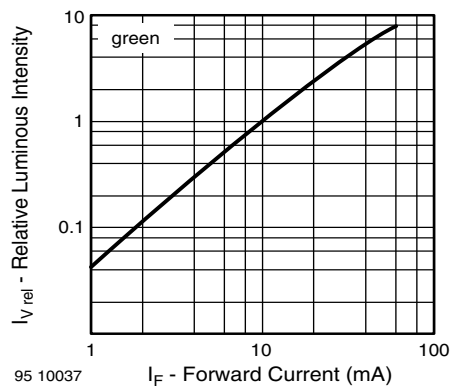
Fig. 20 - Relative Luminous Intensity vs. Forward Current
