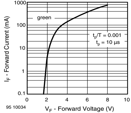
Fig. 19 - Forward Current vs. Forward Voltage
