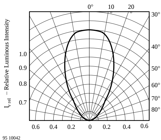
Figure 19 Rel. Luminous Intensity vs. Angular Displacement
