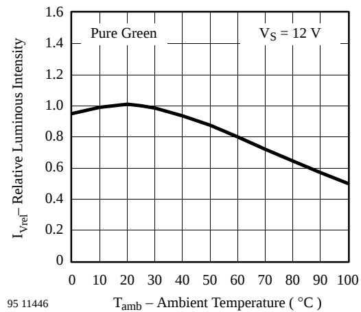
Figure 29 Rel. Luminous Intensity vs. Ambient Temperature
