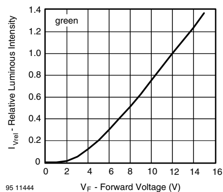
Fig. 21 - Relative Luminous Intensity vs. Forward Voltage
