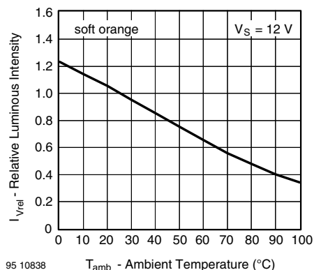
Fig. 11 - Relative Luminous Intensity vs. Ambient Temperature
