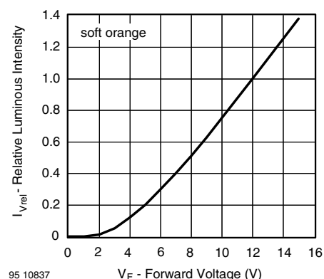
Fig. 10 - Relative Luminous Intensity vs. Forward Voltage
