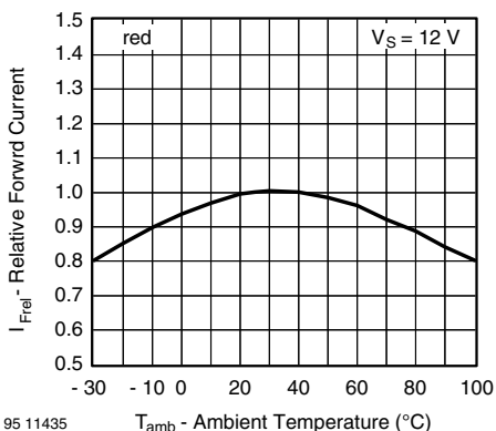
Fig. 2 - Relative Forward Current vs. Ambient Temperature
