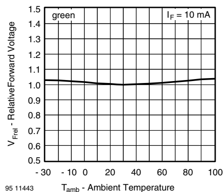
Fig. 20 - Relative Forward Voltage vs. Ambient Temperature
