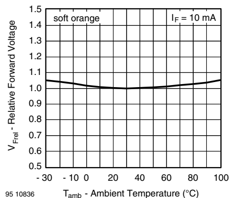
Fig. 9 - Relative Forward Voltage vs. Ambient Temperature
