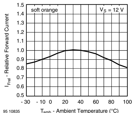
Fig. 8 - Relative Forward Current vs. Ambient Temperature
