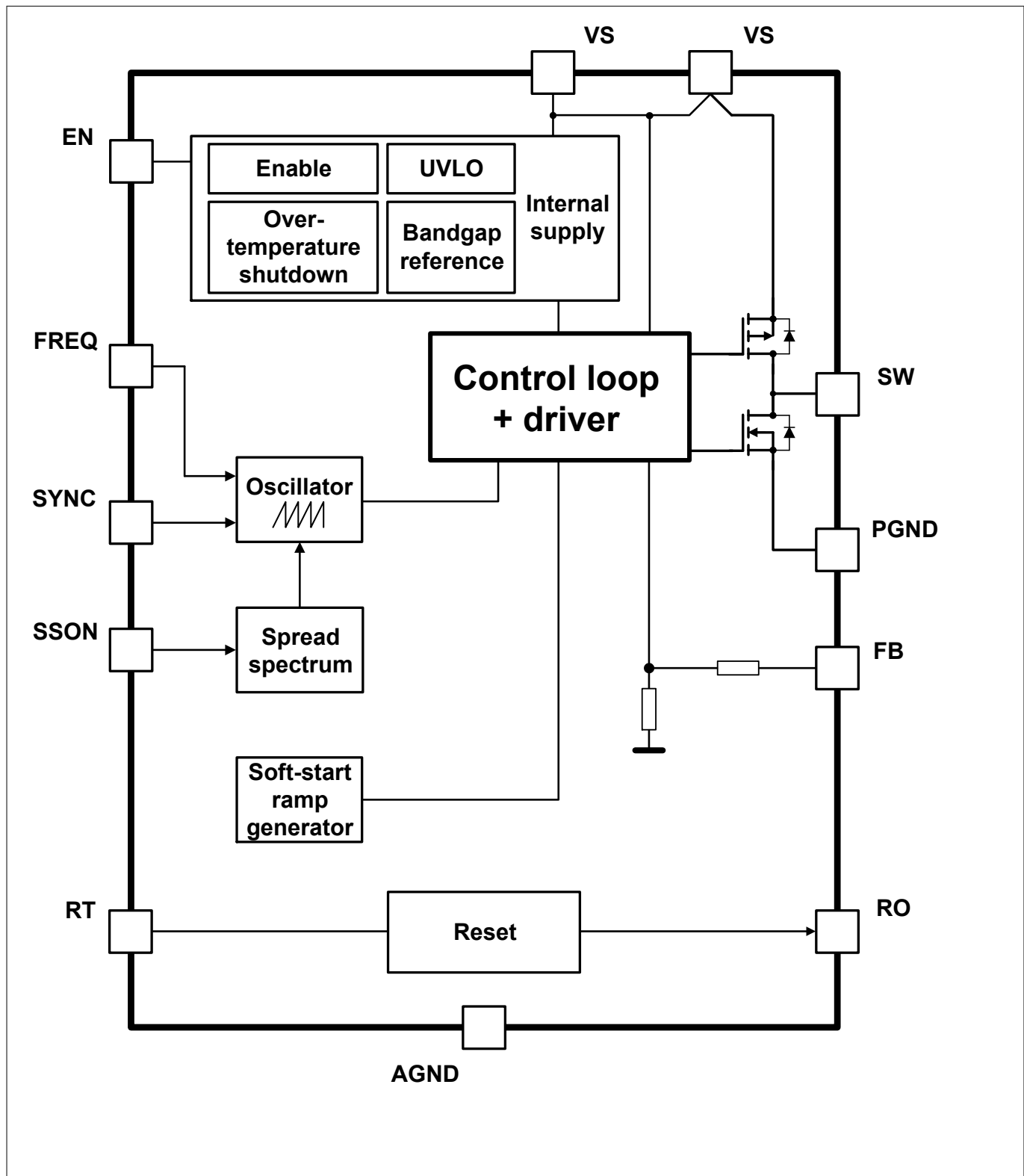
Figure 1 Block diagram
