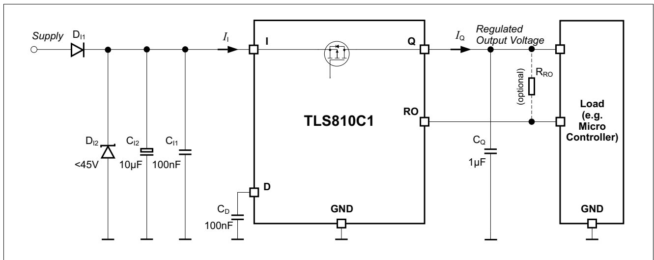
Figure 6 Application Diagram TLS810C1
