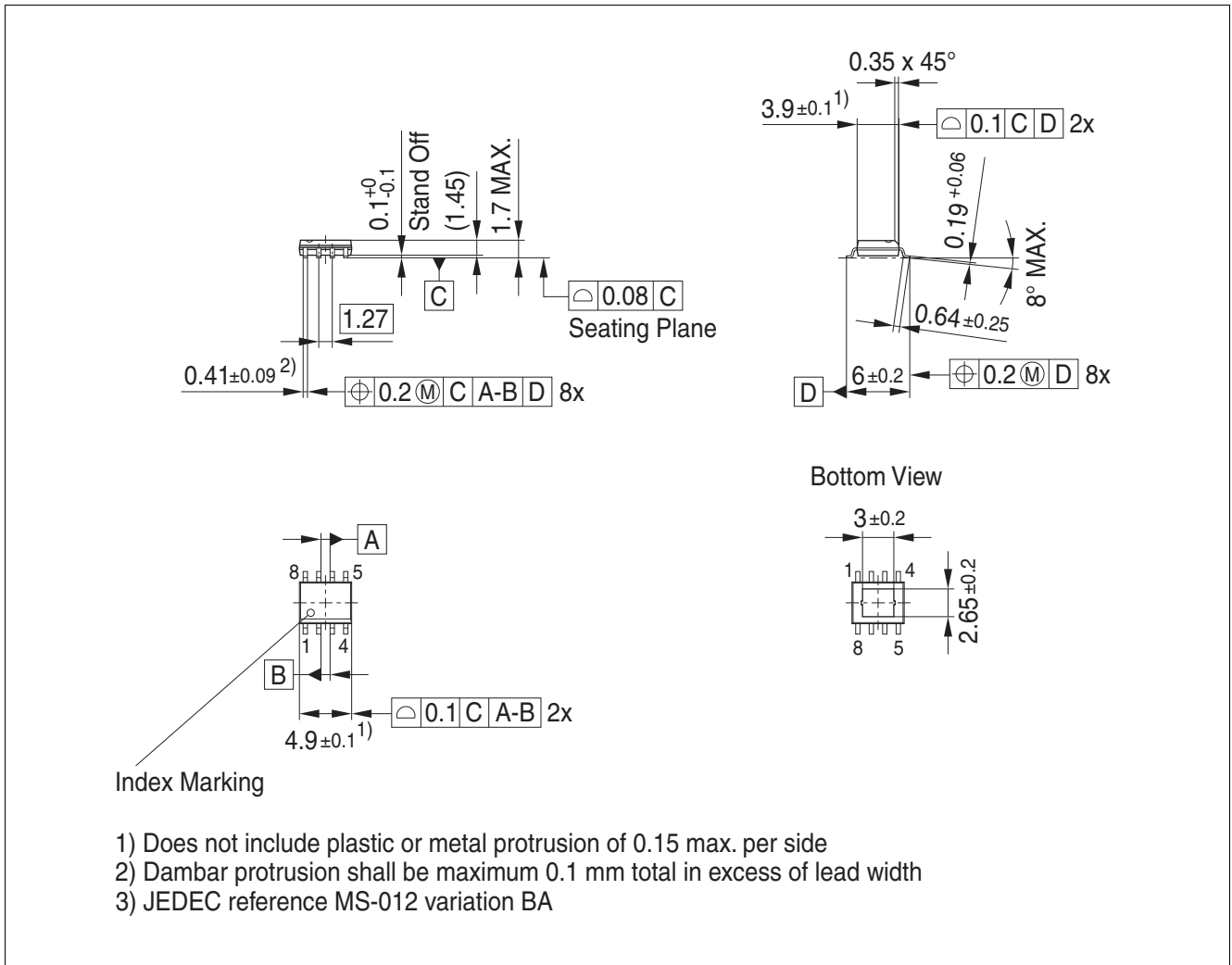
Figure 7 PG-DSO-8 EP
