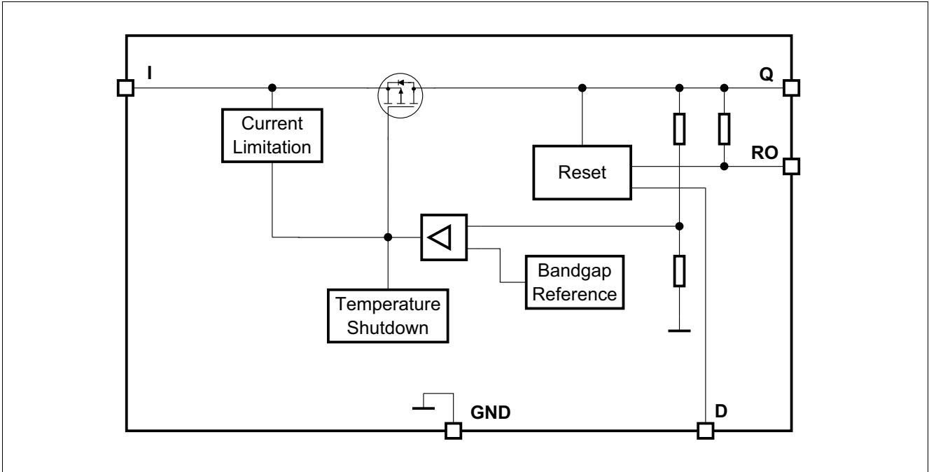
Figure 1 Block Diagram TLS810C1
