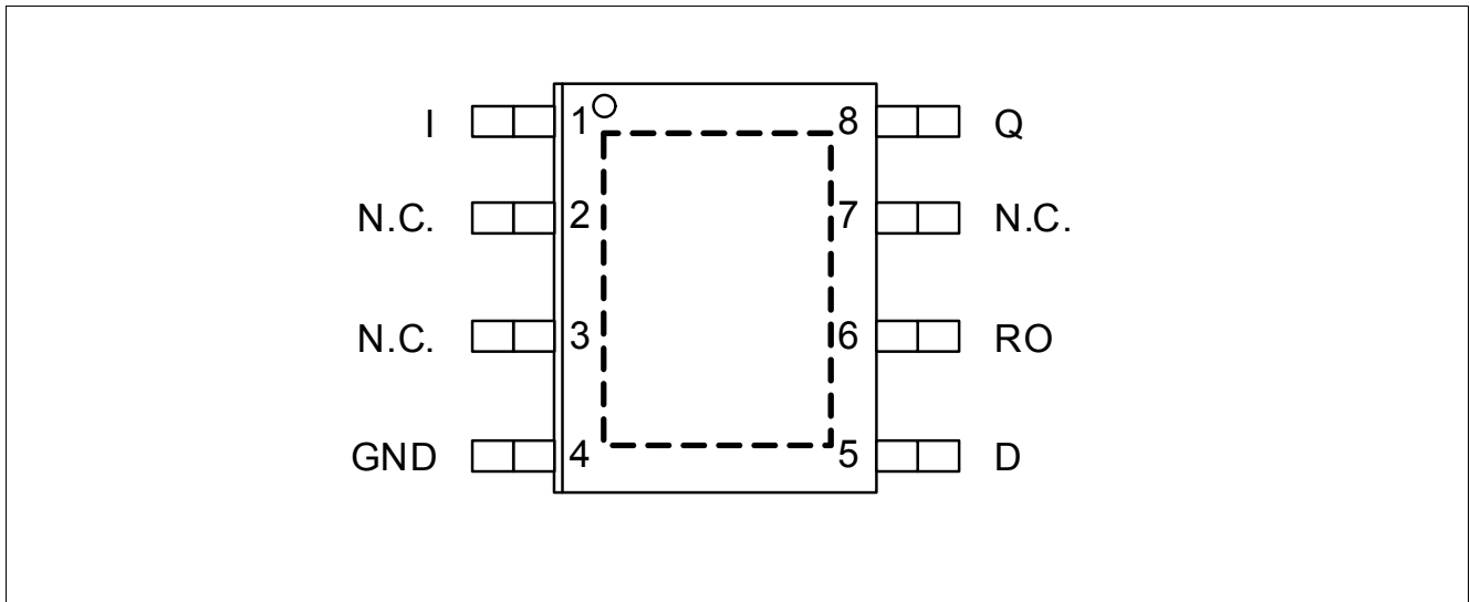
Figure 2 Pin Configuration TLS810C1 in PG-DSO-8 EP package
