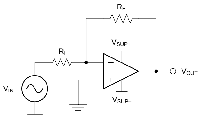
Figure 34. Amplifier Schematic
