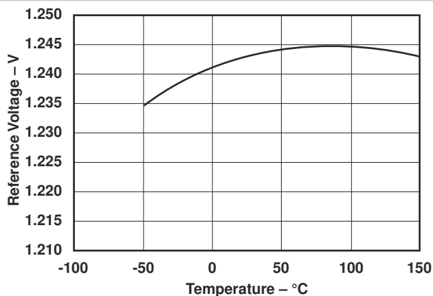
Figure 7-18. Reference Voltage vs Temperature
