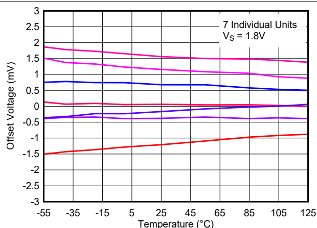
Figure 8-26. Offset Voltage vs. Temperature, 1.8 V
