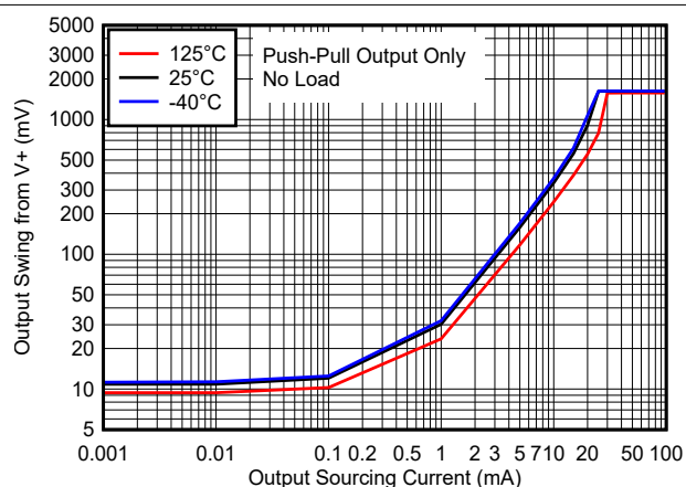
Figure 8-2. Output Swing vs. Output Sourcing Current - 1.8V
