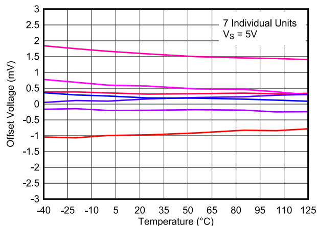
Figure 8-28. Offset Voltage vs. Temperature, 5 V
