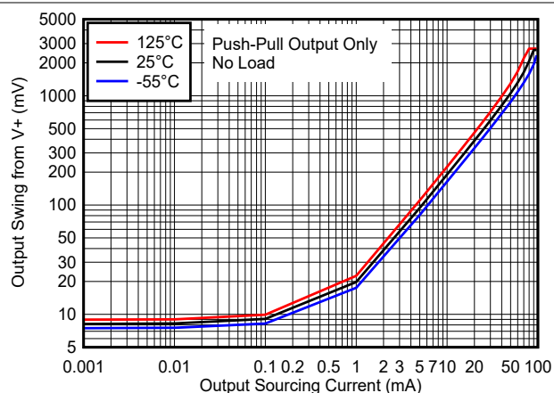
Figure 8-4. Output Swing vs. Output Sourcing Current - 3.3V
