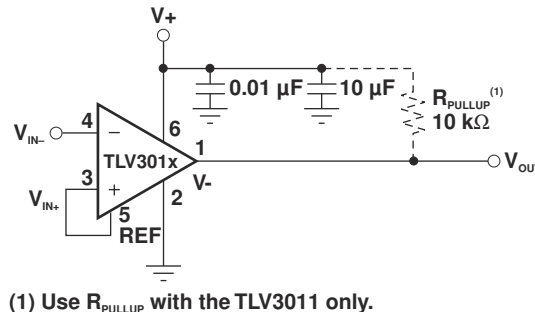
Figure 10-1. Basic Connections
