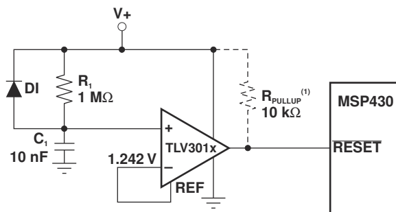
Figure 10-5. TLV3012 Configured as Power-Up Reset Circuit for the MSP430™ Microcontroller
