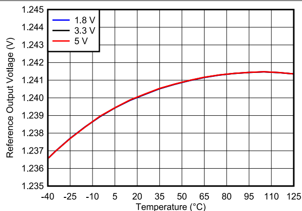
Figure 8-16. Reference Voltage vs. Temperature
