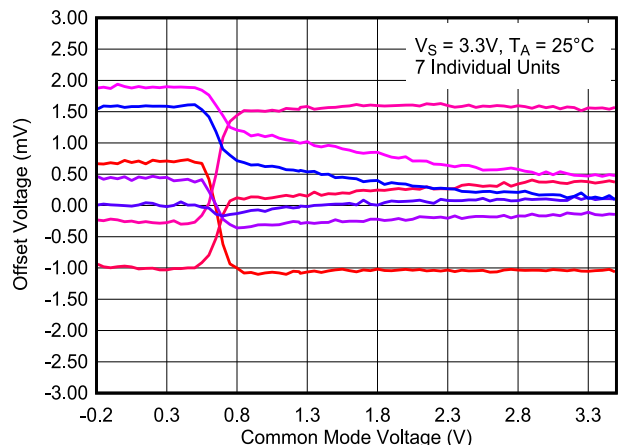
Figure 8-30. Offset Voltage vs. Common Mode Voltage, 3.3 V
