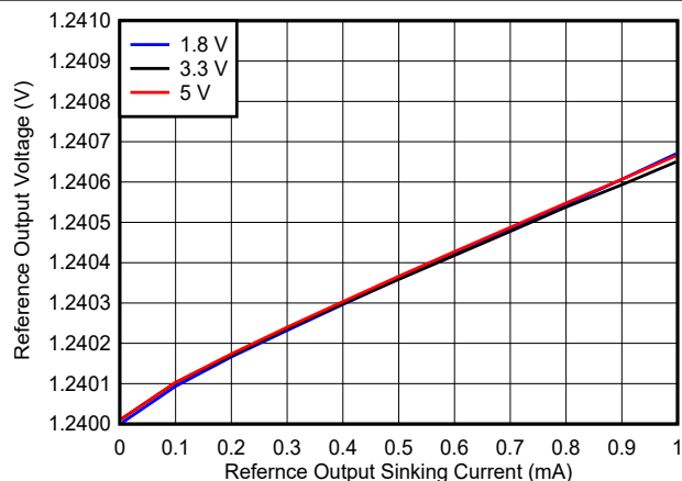
Figure 8-18. Reference Voltage vs. Reference Output Sinking Current
