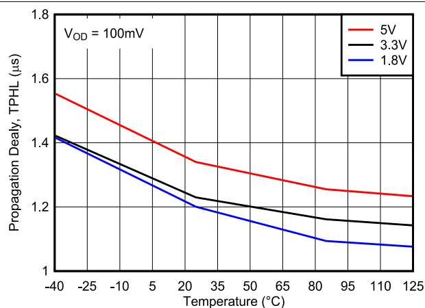
Figure 8-14. High to Low Propagation Delay vs. Temperature
