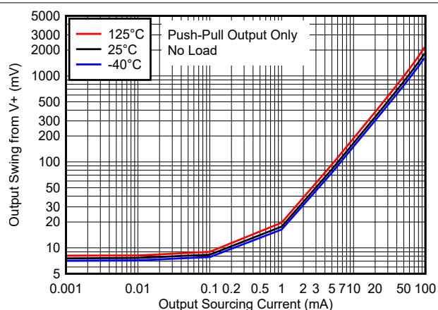
Figure 8-6. Output Swing vs. Output Sourcing Current - 5V
