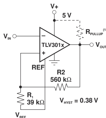
Figure 10-2. Adding Hysteresis
