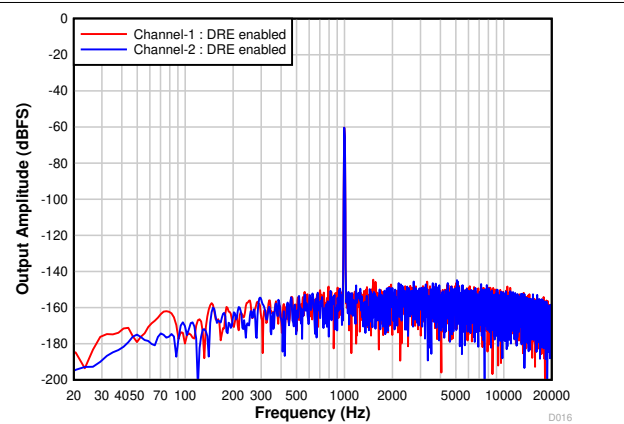
Figure 7-19. FFT With a -60-dB Input With DRE Enabled
