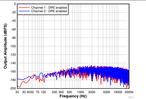
Figure 7-17. FFT With Idle Input With DRE Enabled
