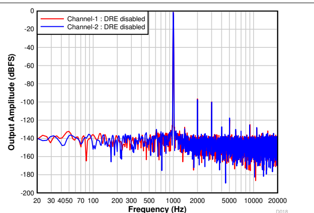
Figure 7-21. FFT With a -1-dB Input With DRE Disabled
