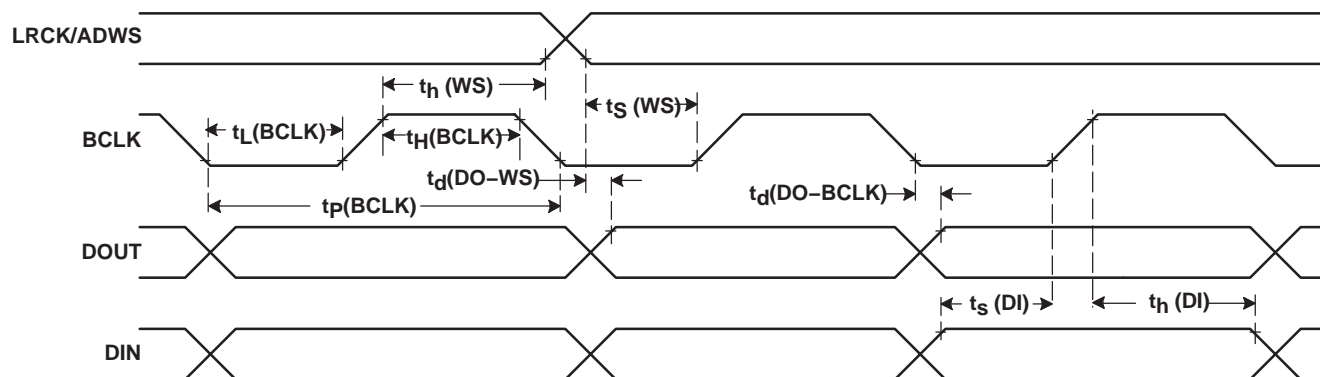
Figure 3. I²S/LJF/RJF Timing in Slave Mode
