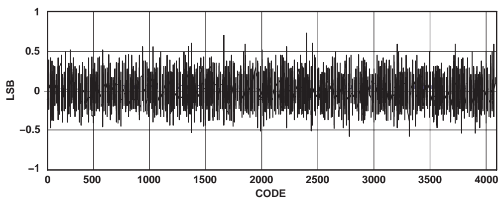
Figure 6. SAR DNL ( T_A = 25^\circ\text{C} , Internal Ref = 2.5 V, AVDD = 3.3 V)
