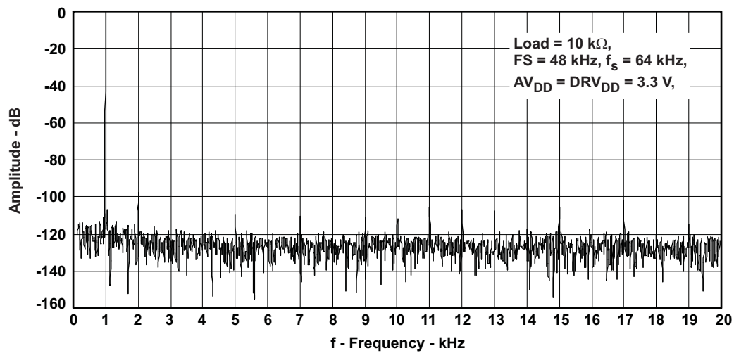
Figure 10. Right-DAC FFT
