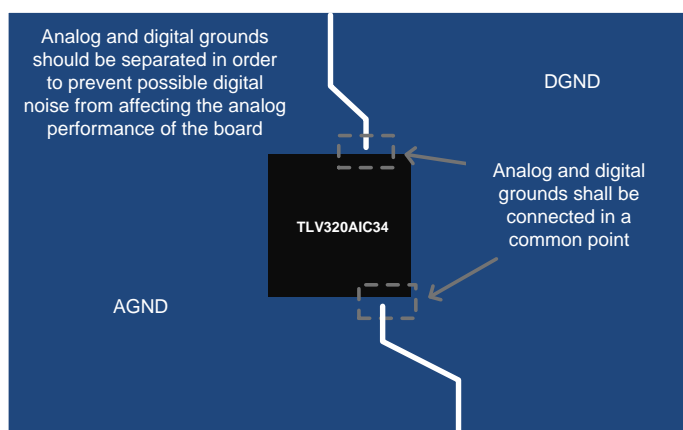
Figure 42. Ground Layer
