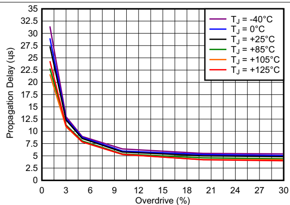
Figure 17. Propagation Delay vs Overdrive ( V+ = 5.5\text{ V} )
