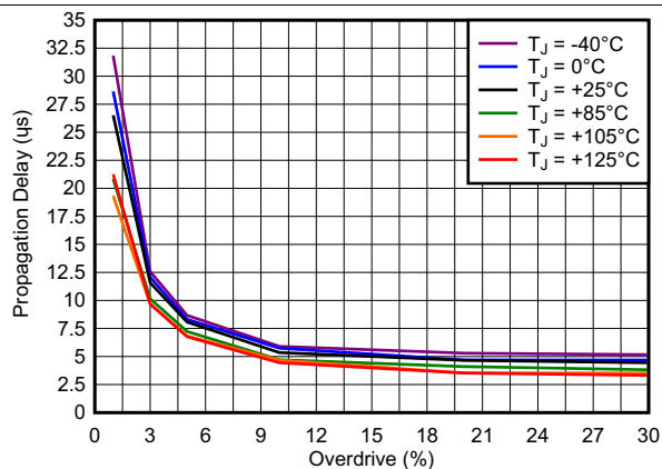
Figure 16. Propagation Delay vs Overdrive ( V+ = 1.5\text{ V} )
