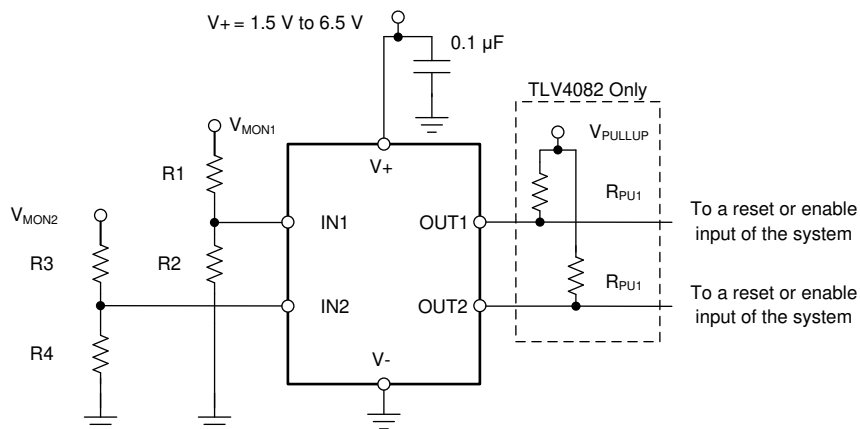
Figure 23. Monitoring Two Separate Rails Schematic
