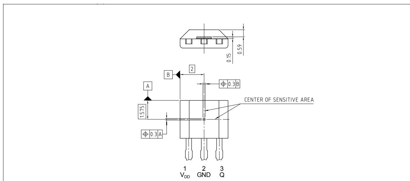
Figure 2 Pin Configuration and Center of Sensitive Area
