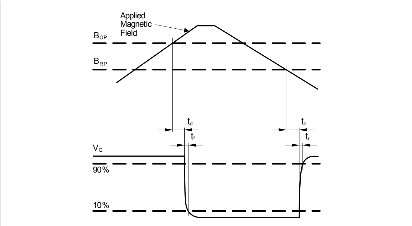
Figure 4 TLV4961-1T
