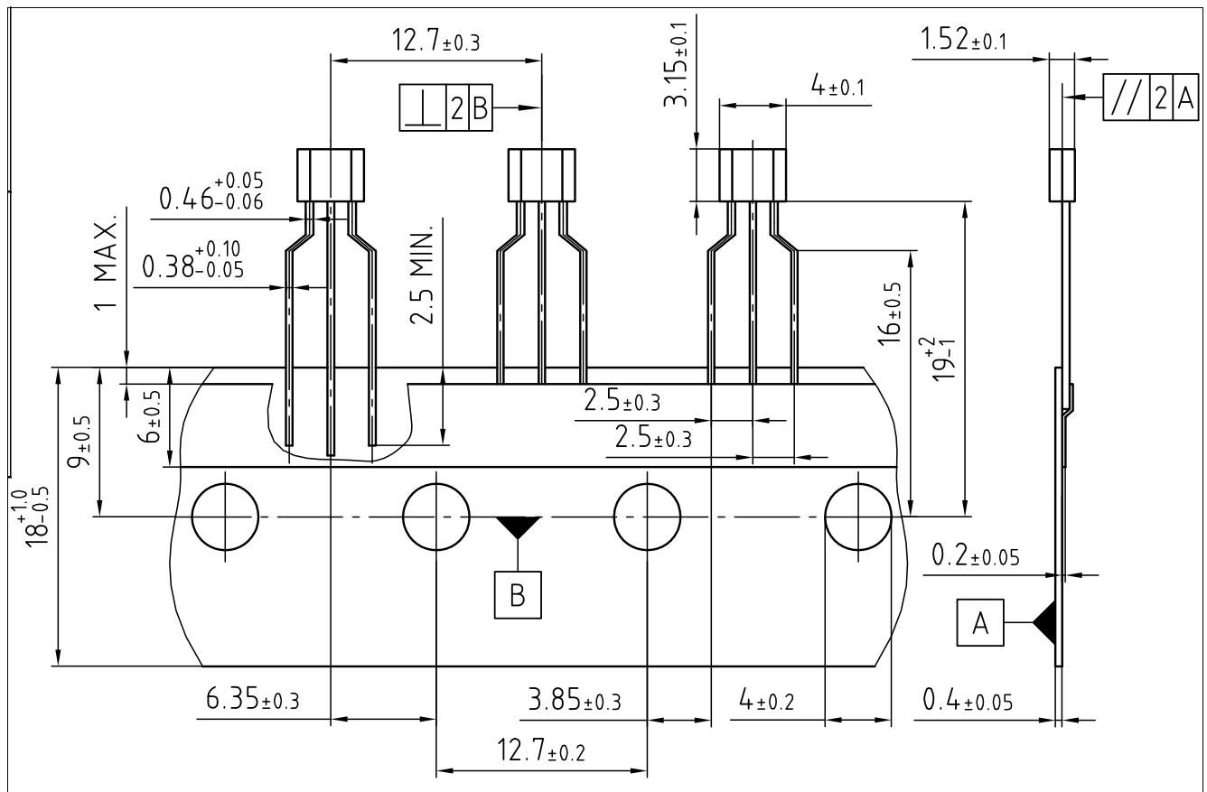
Figure 12 Packing of the TLV4961-1TB TO92S-3-2
