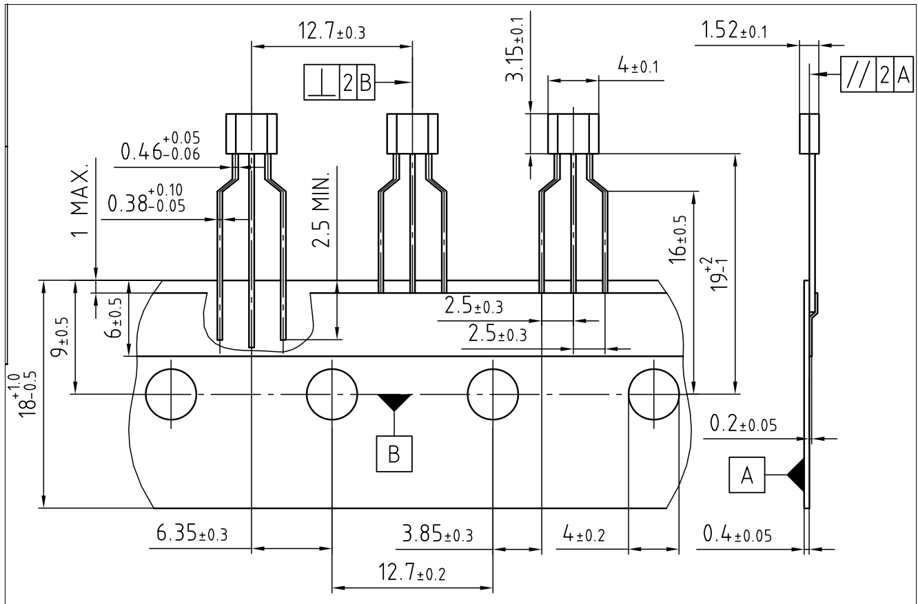
Figure 12 Packing of the TLV4968-1TB T092S-3-2
