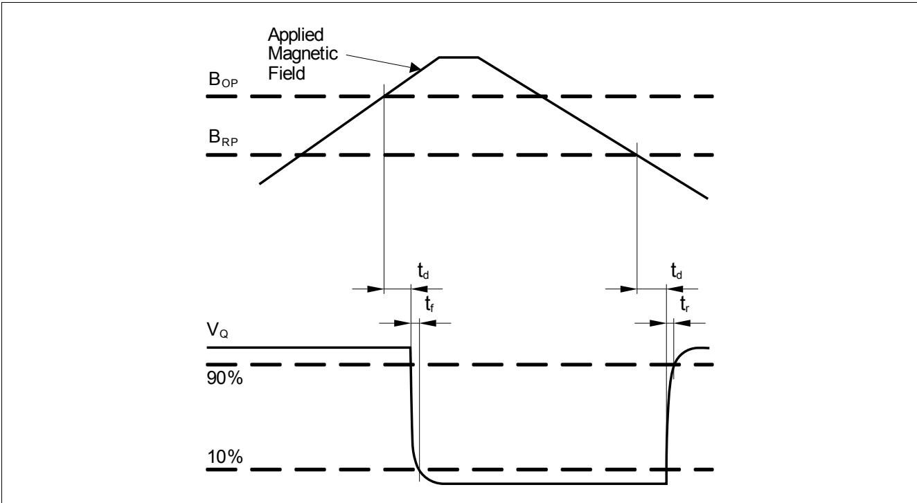
Figure 4 TLV4968-1T
