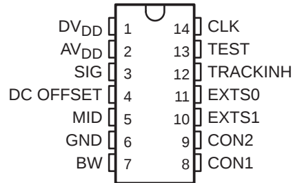
D PACKAGE (TOP VIEW)
