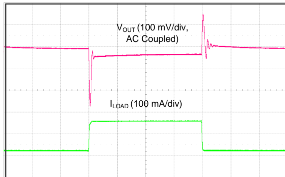
Time (20 \mu\text{s}/\text{div} ) V_{IN} = 3.8\text{ V} , 1- \mu\text{F} output capacitor, output current slew rate = 0.25\text{ A}/\mu\text{s}
