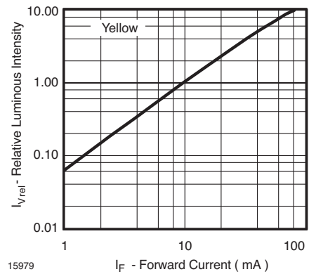
Figure 15. Relative Luminous Flux vs. Forward Current
