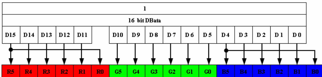
16-bit Data Bus GRAM Write/Read Data Format (16bit, 65k)
