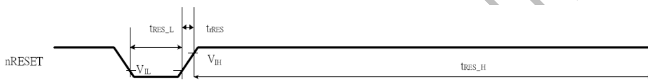
Figure 5.2 RESET Timing
