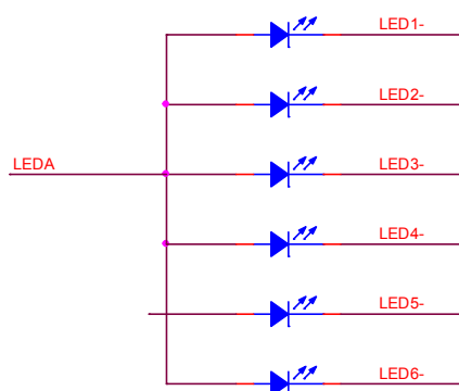
Figure 4.2 LED driver circuit
