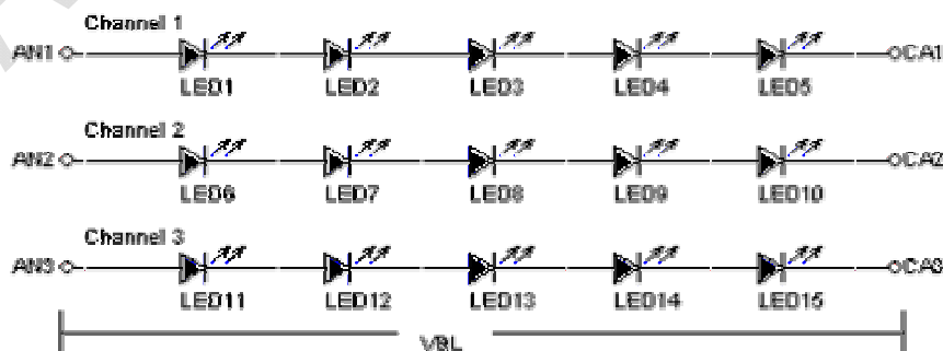
Figure 4.2 LED connection of backlight
