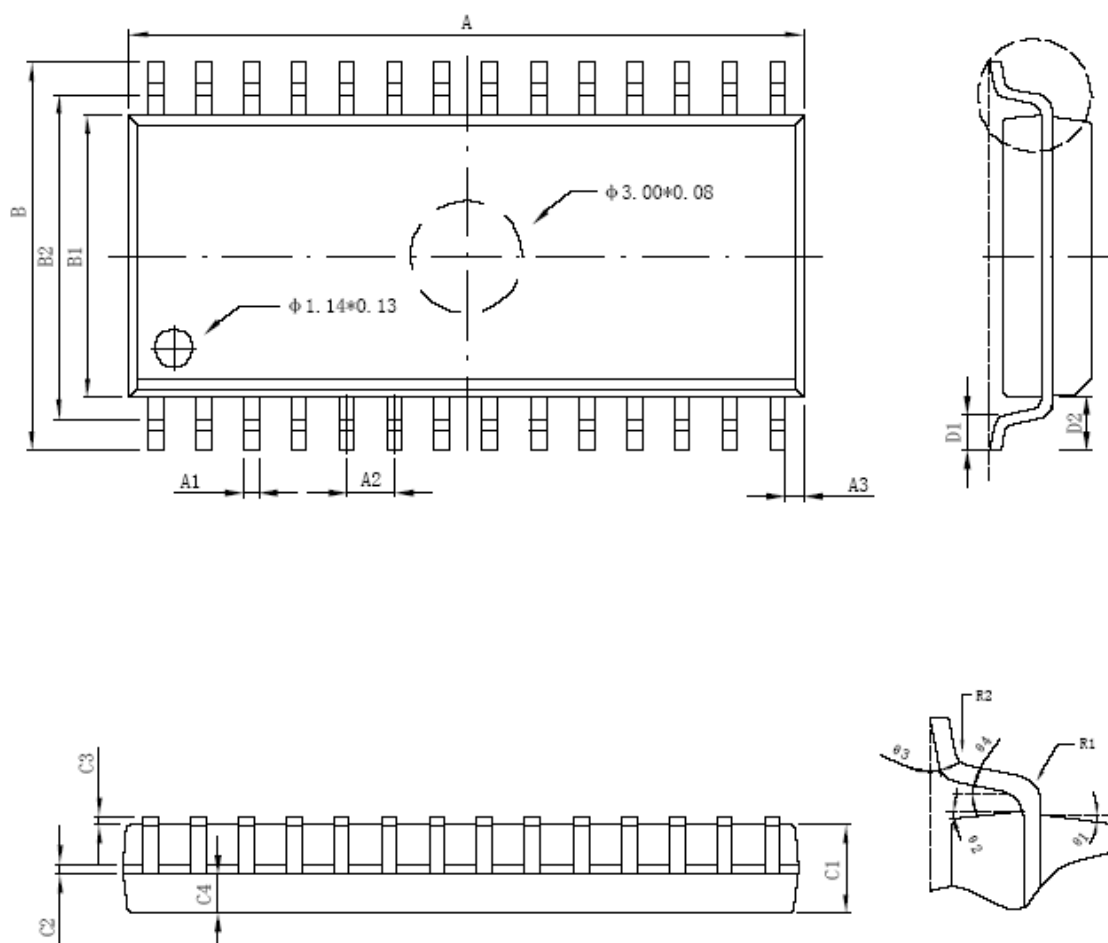
DETAIL "X"
