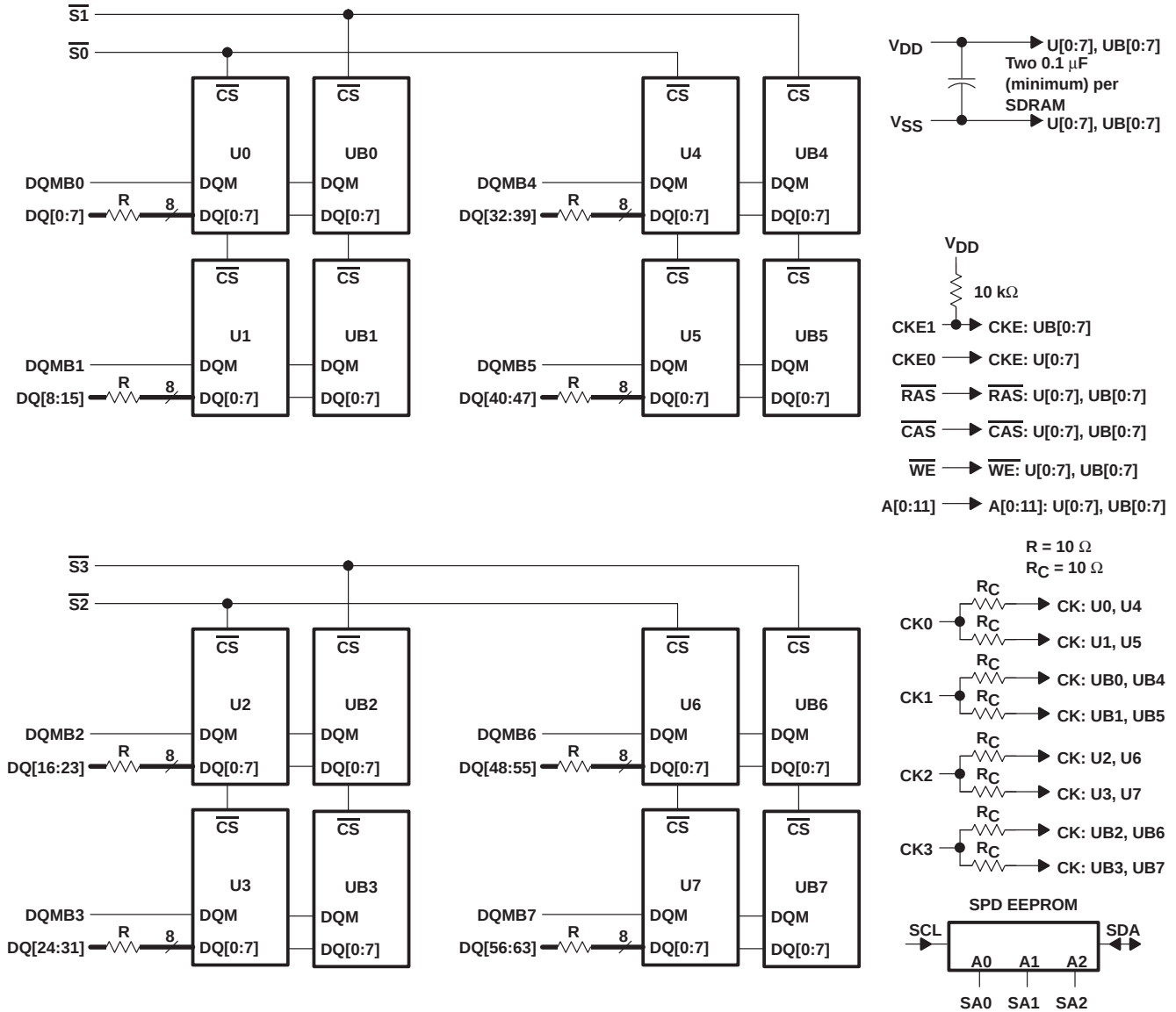
functional block diagram for the TM4SN64EPH
