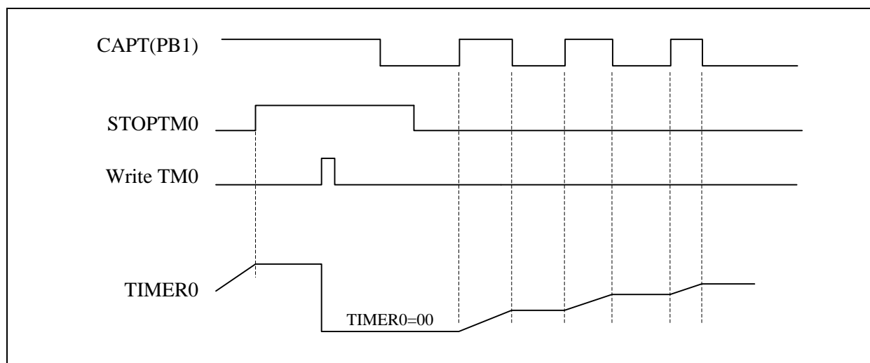
Figure 3.5.2 Timer0 is used to measure the high (or low) time on CAPT pin
