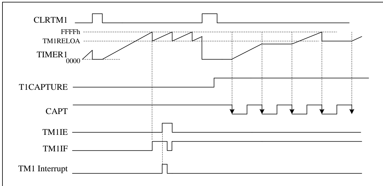
Figure 3.3.2 (CAPOLARITY=0, implies CAPT falling edge)
