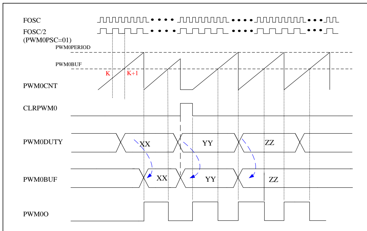
Figure 3.6.3 PWM0 Timing (CLR PWM0 after PWM0CNT over PWM0BUF)
