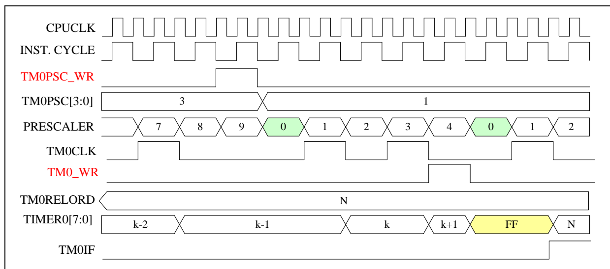
Figure 3.2.2 Timer0 works in timer mode
