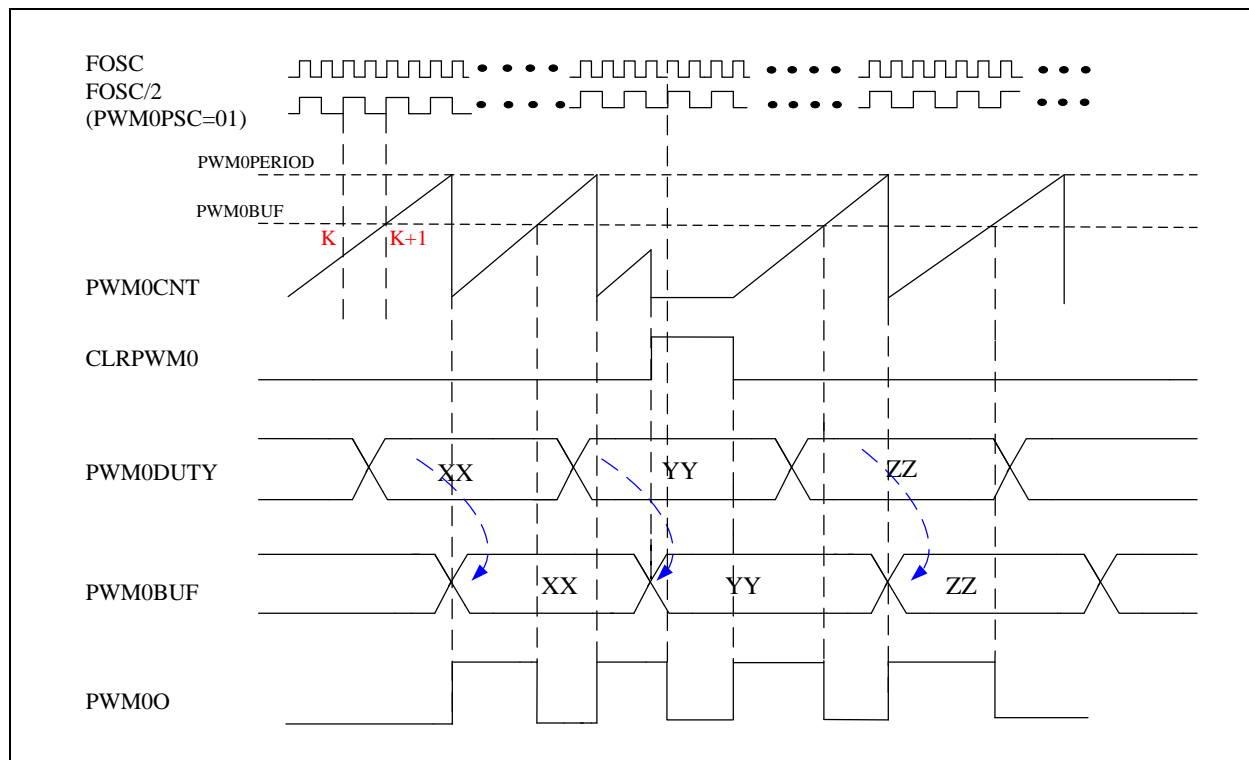
Figure 3.6.2 PWM0 Timing (CLR PWM0 before PWM0CNT reaches PWM0BUF)
