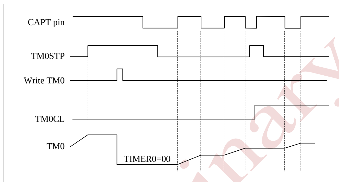
Timer0 is used to measure the high (or low) time on CAPT pin
