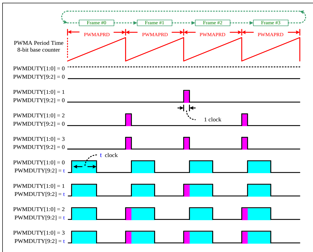
PWM Timing Diagram
