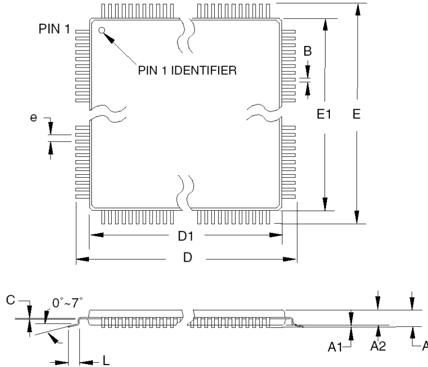
Figure 6.1: Package Outline
