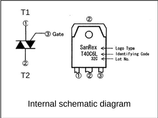
Non-isolated TO-3P Package
