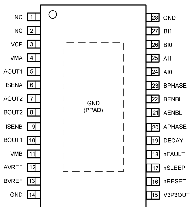
HTSSOP28(Top view)
