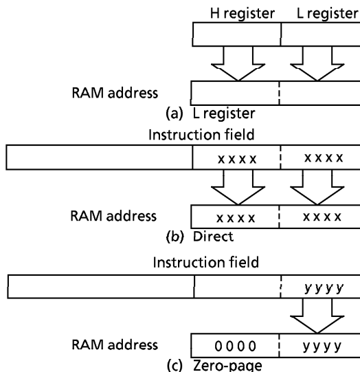
Figure 2-5. Addressing mode
