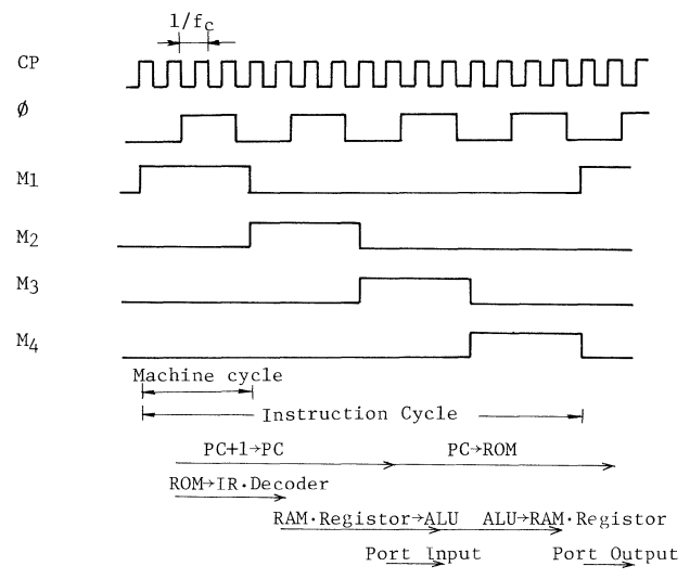
Fig. 2.1.1 Instruction Cycle
