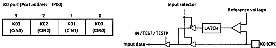
Figure 3-1. Port K0
