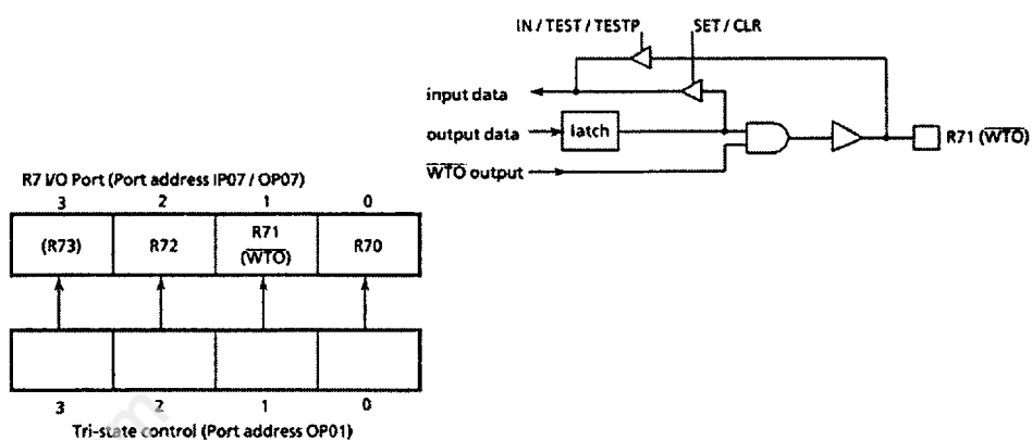
Figure 3-3. Port R7
