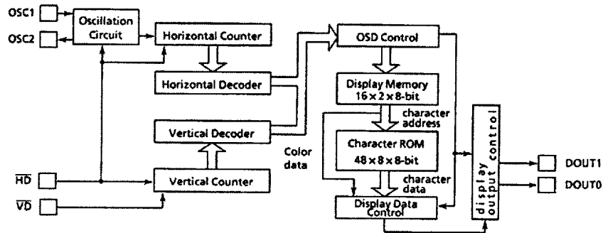
Figure 3-6. OSD Circuit
