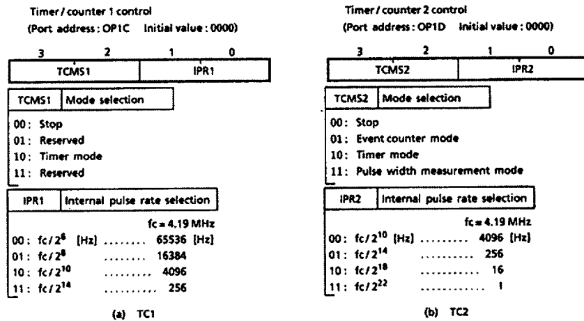
Figure 3-5. Timer/Counter Control Command Registers
