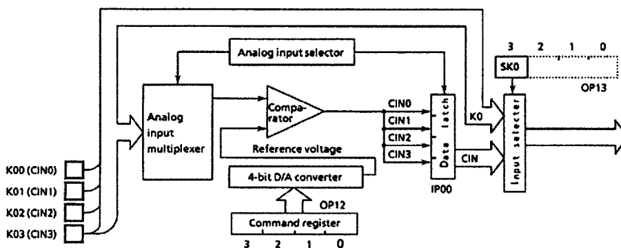
Figure 3-11. Circuit of Comparator Input
