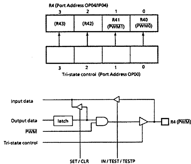
Figure 3-2. Port R4 (PWM)
