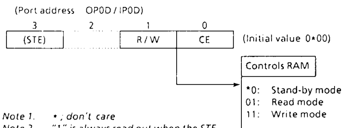
Figure 2-4. RAM Command Register
