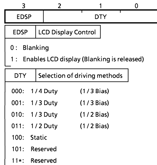
Figure 2-9. LCD Driver control Command Register
