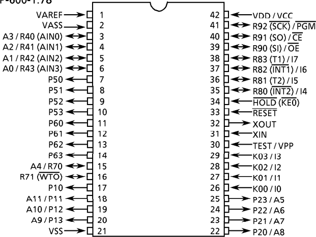
SDIP42-P-600-1.78
