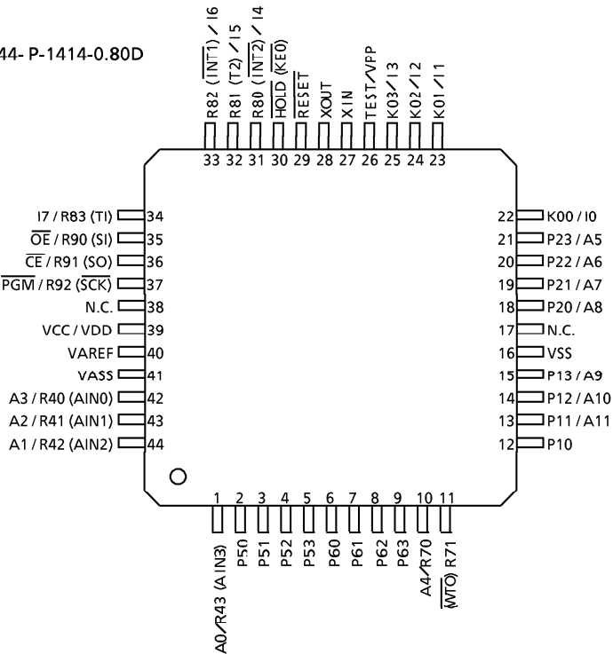
QFP44- P-1414-0.80D
