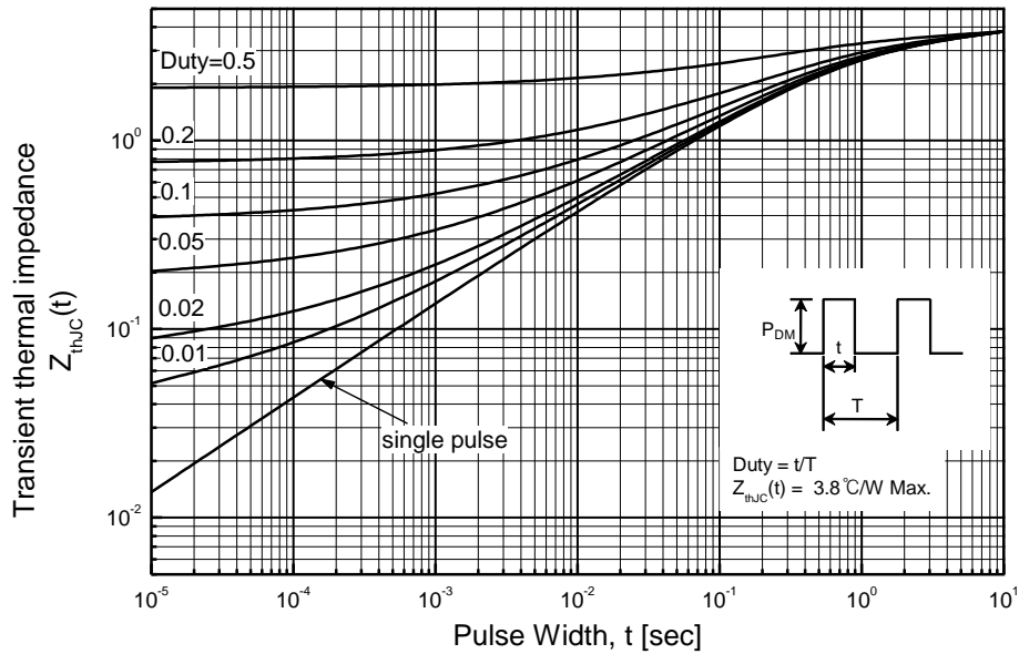
TMPF5N60Z(G)
