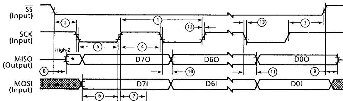
(f) SPI Slave Timing CPOL = 1, CPHA = 1
