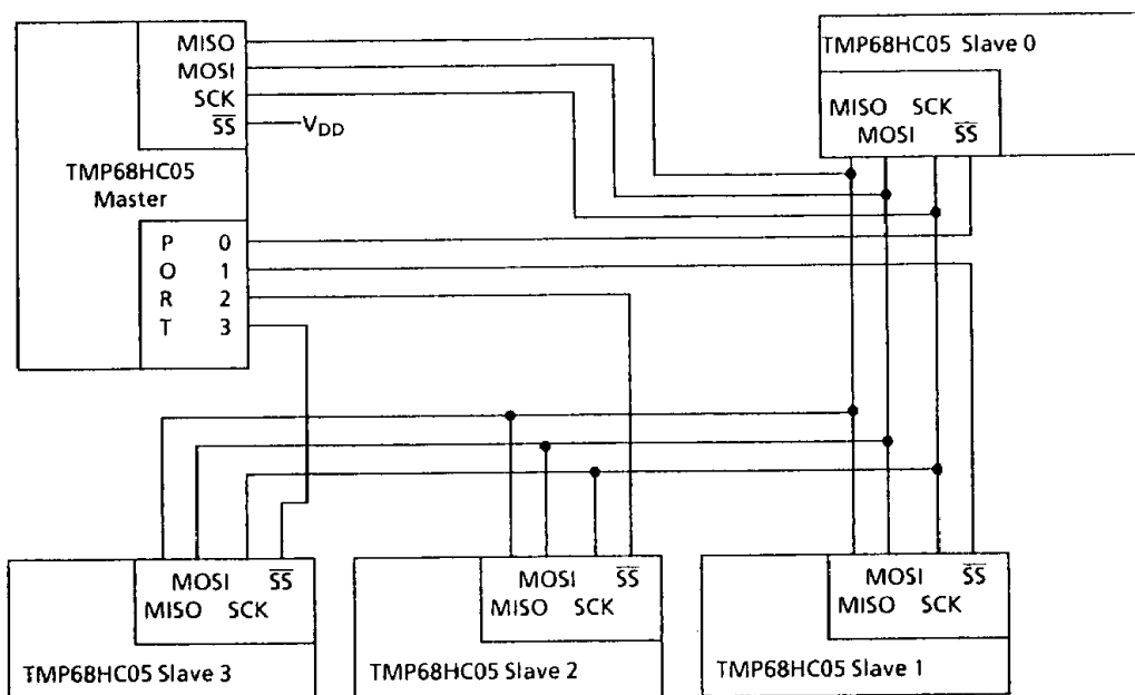
a. Single Master, Four Slaves
