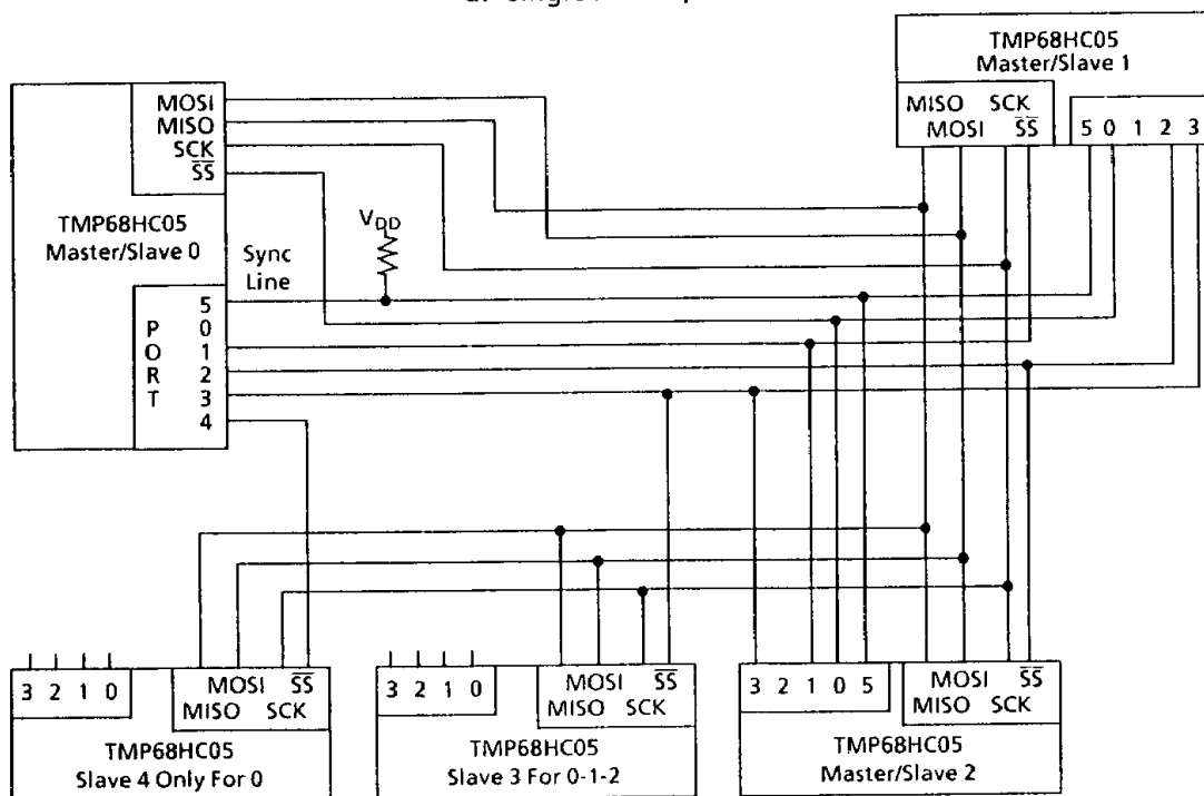
b. Three Master/Slave, Two Slaves
