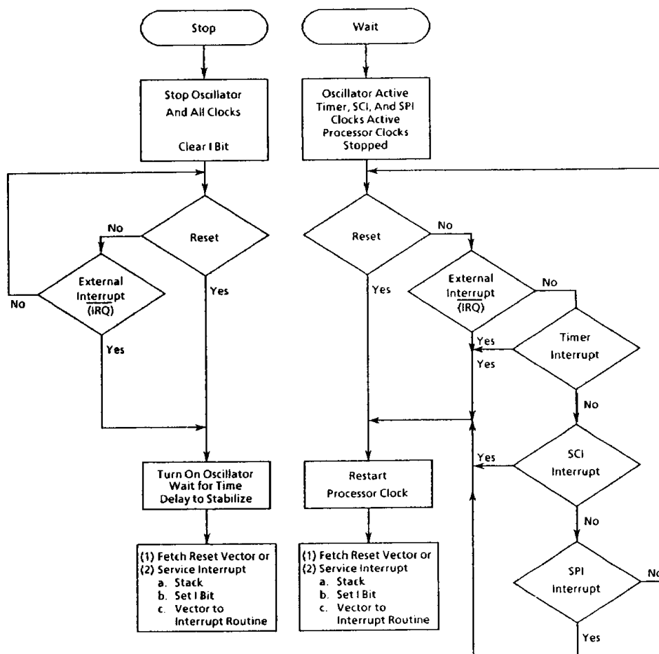
Figure 3.3 STOP/WAIT Flowcharts
