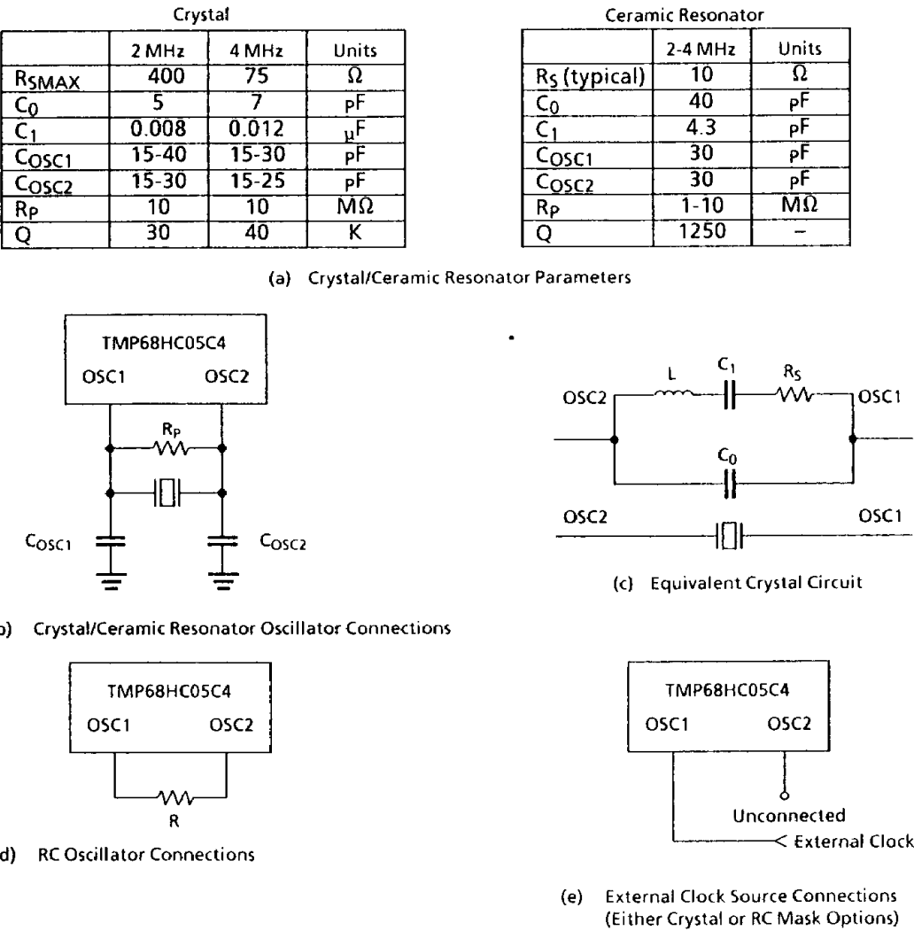
Figuer 2.1 Oscillator Connections
