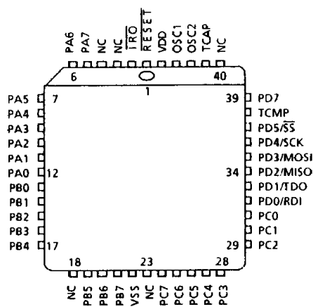
T SUFFIX 44-Lead PLCC Package
