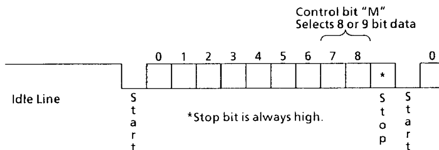
Figure 5.1 Data Format
