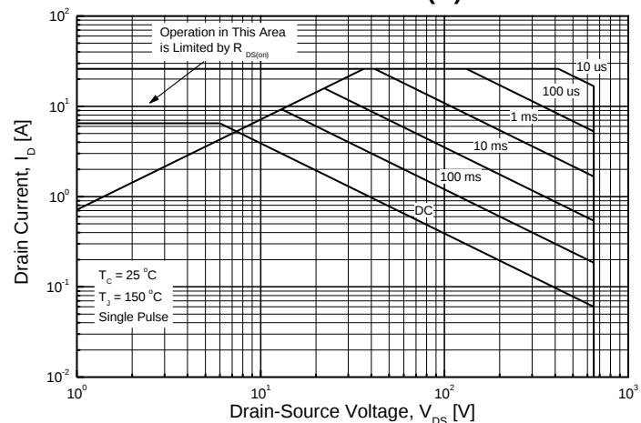
TMPF7N65AZ(G)
