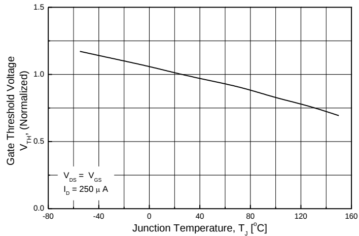
TMPF7N65AZ(G)
