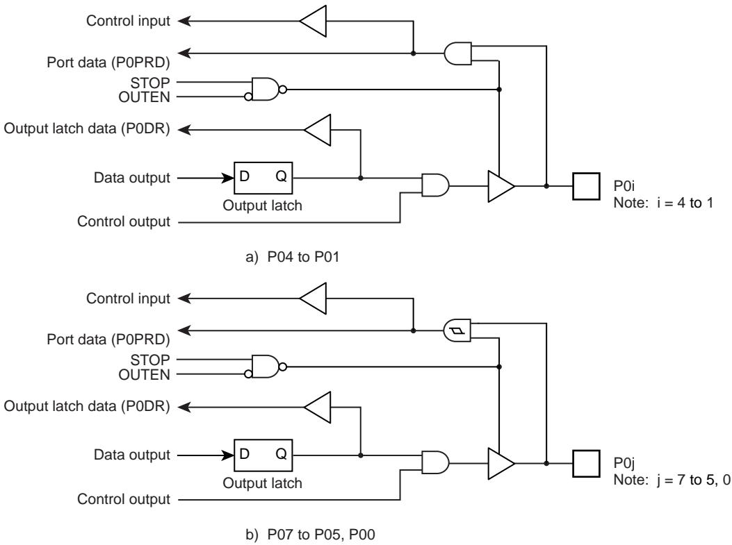
Figure 5-2 Port 0
