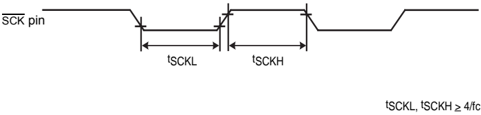
Figure 9-3 External Clock
