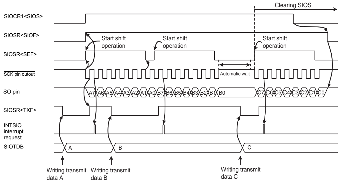
Figure 9-6 Example of Internal Clock and MSB Transmit Mode
