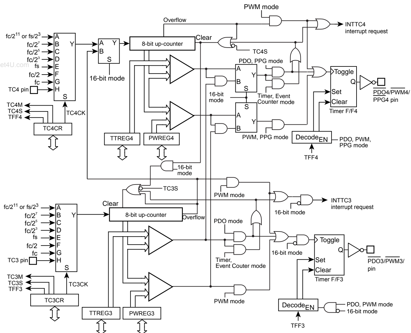
Figure 8-1 8-Bit TimerCounter 3, 4
