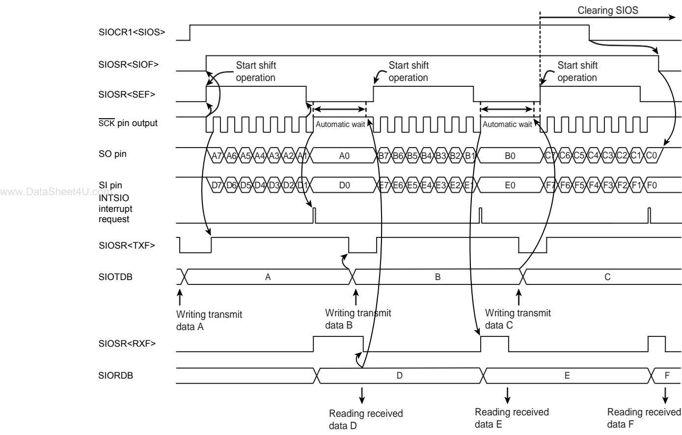
Figure 9-13 Example of Internal Clock and MSB Transmit/Receive Mode
