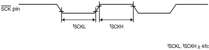
Figure 10-3 External Clock
