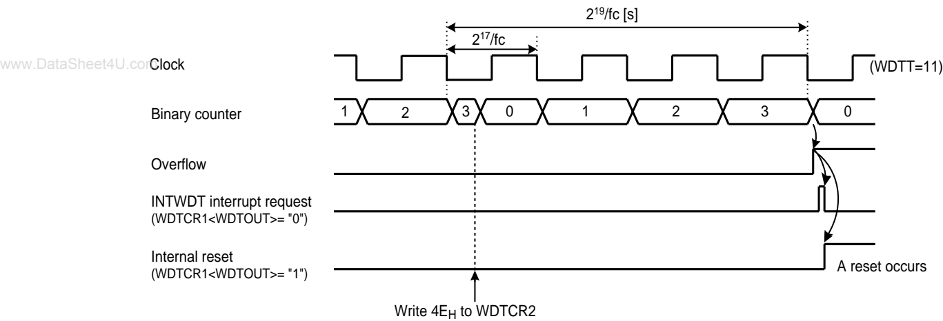
Figure 6-2 Watchdog Timer Interrupt
