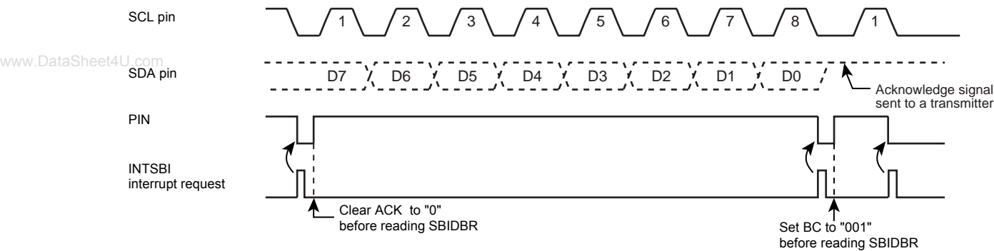
Figure 16-12 Termination of Data Transfer in Master Receiver Mode
