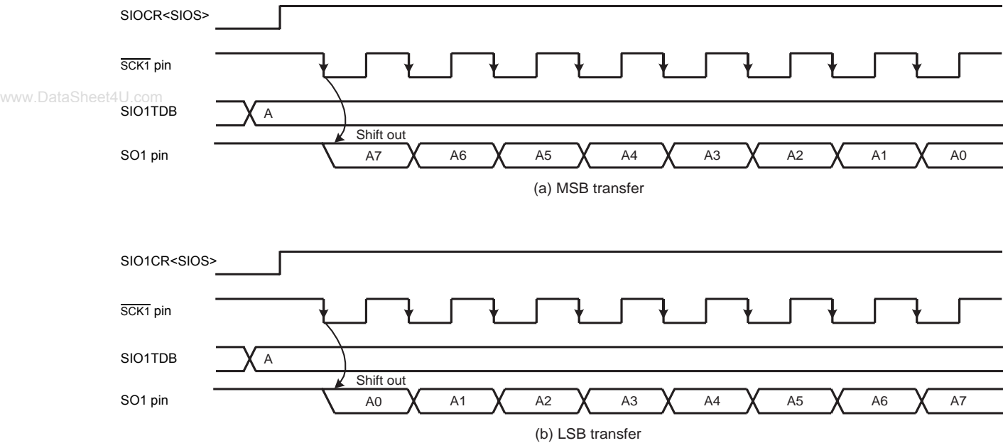
Figure 14-5 Transfer Bit Direction (Example of transmit mode)
