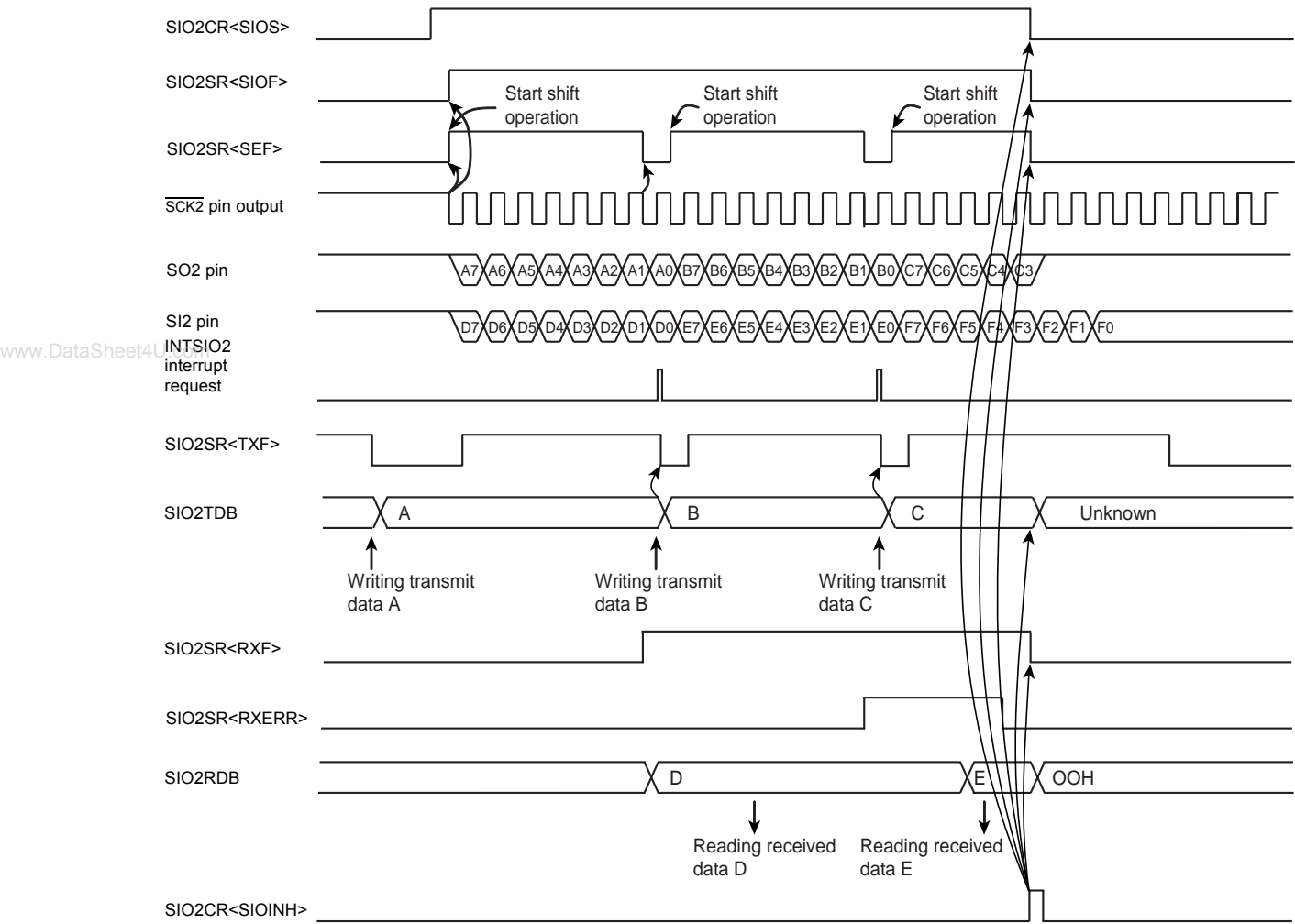
Figure 15-16 Example of Transmit/Receive (Receive) Error Processing
