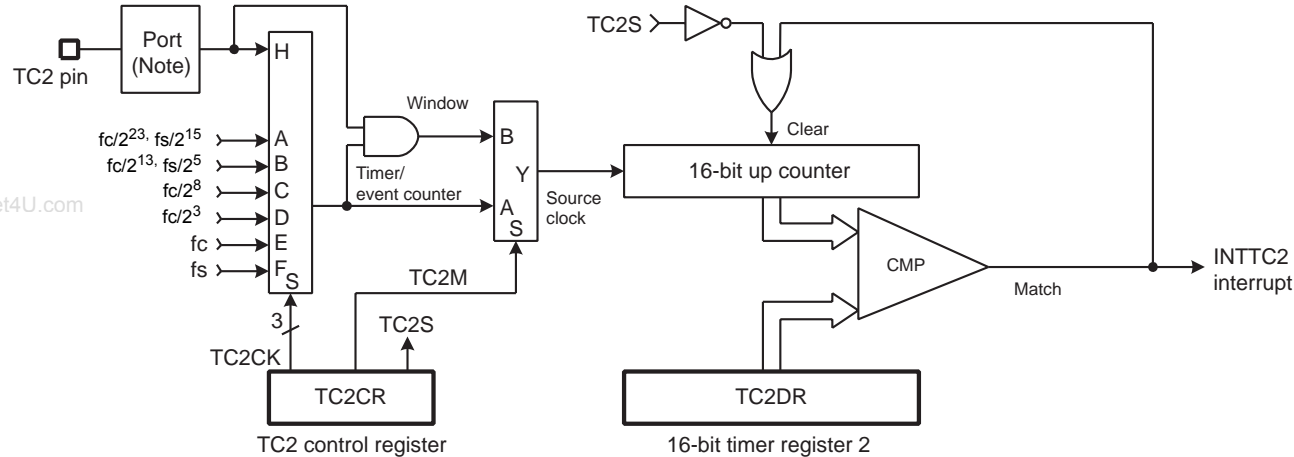
Figure 9-1 Timer/Counter2 (TC2)
