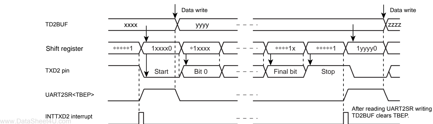
Figure 13-9 Generation of Transmit Data Buffer Empty
