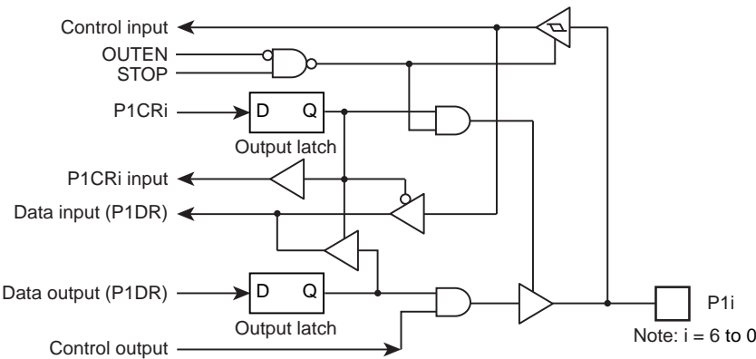
Figure 5-3 P1 Port
