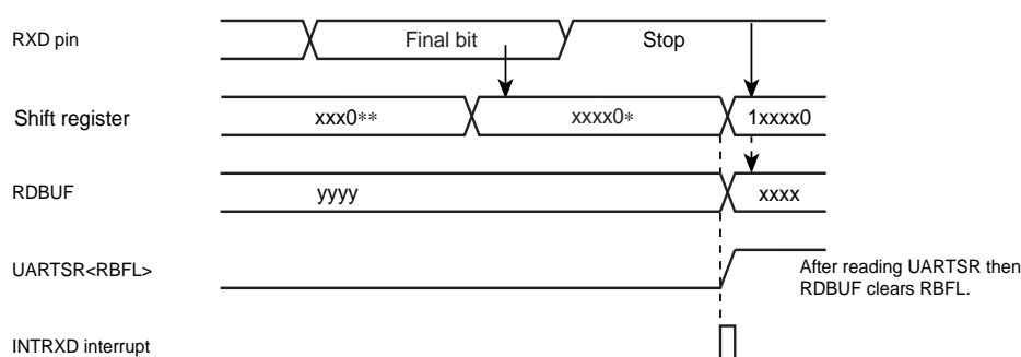
Figure 10-8 Generation of Receive Data Buffer Full
