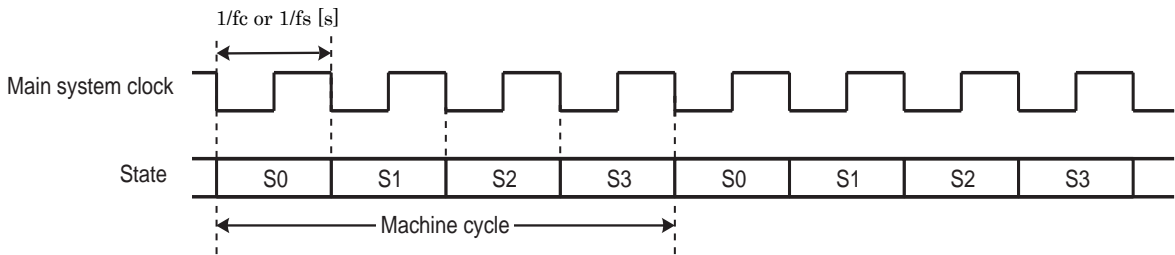
Figure 2-5 Machine Cycle
