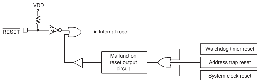
Figure 2-15 Reset Circuit
