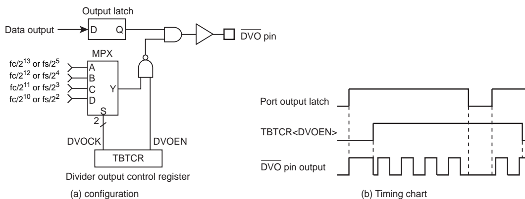
Figure 6-3 Divider Output
