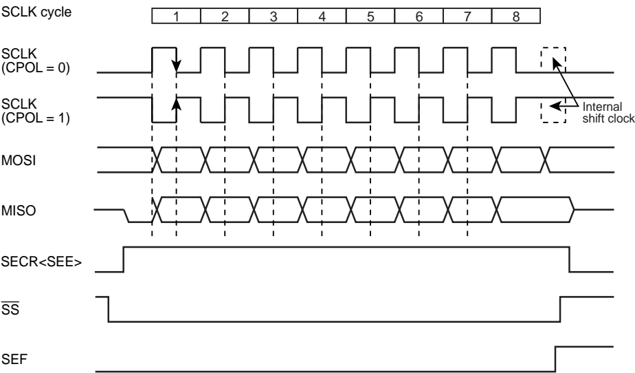
Figure 11-3 Transfer Format where CPHA = 1
