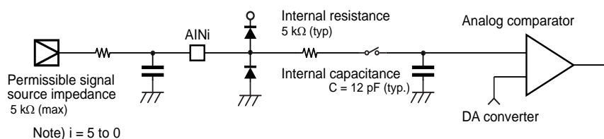
Figure 12-5 Analog Input Equivalent Circuit and Example of Input Pin Processing
