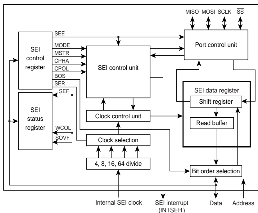
Figure 11-1 SEI (Serial Extended Interface)
