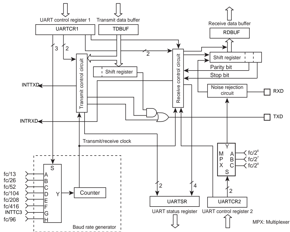
Figure 10-1 UART (Asynchronous Serial Interface)
