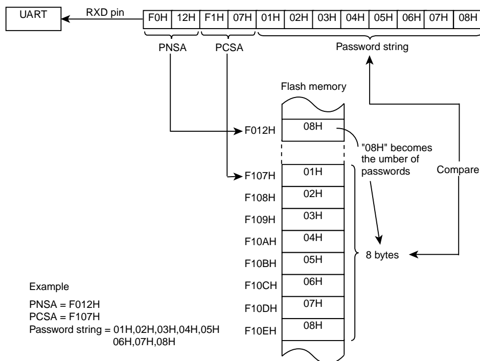
Figure 15-5 Password Comparison
