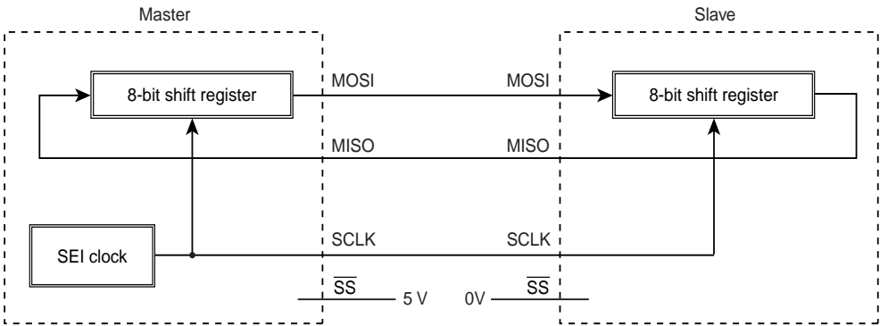
Figure 11-4 Master and Slave Connection in SEI
