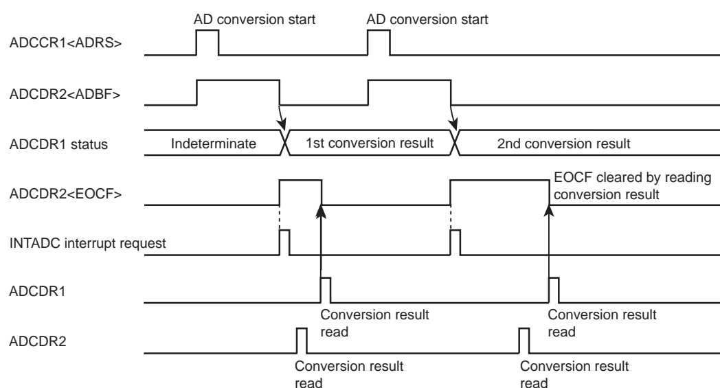
Figure 12-2 Software Start Mode
