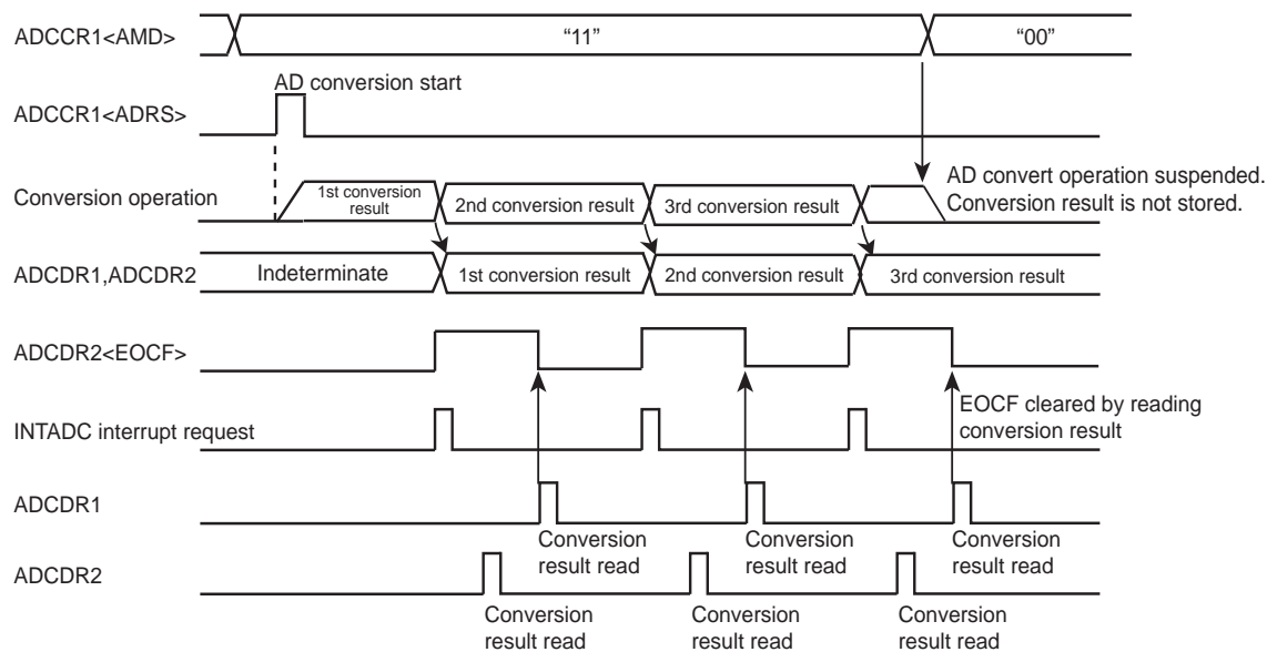
Figure 12-3 Repeat Mode
