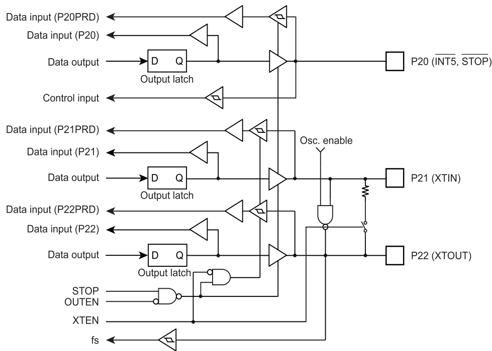
Figure 5-4 P2 Port
