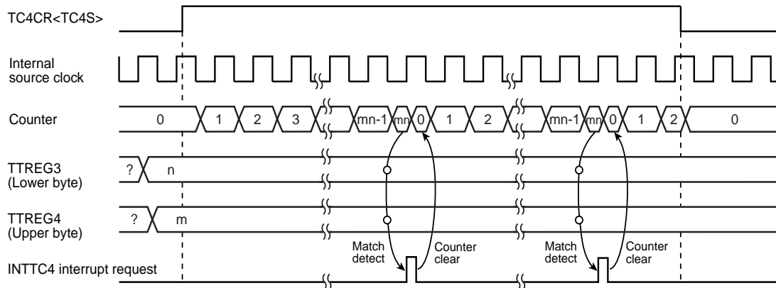
Figure 9-6 16-Bit Timer Mode Timing Chart (TC3 and TC4)
