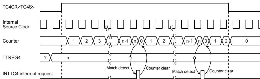
Figure 9-2 8-Bit Timer Mode Timing Chart (TC4)
