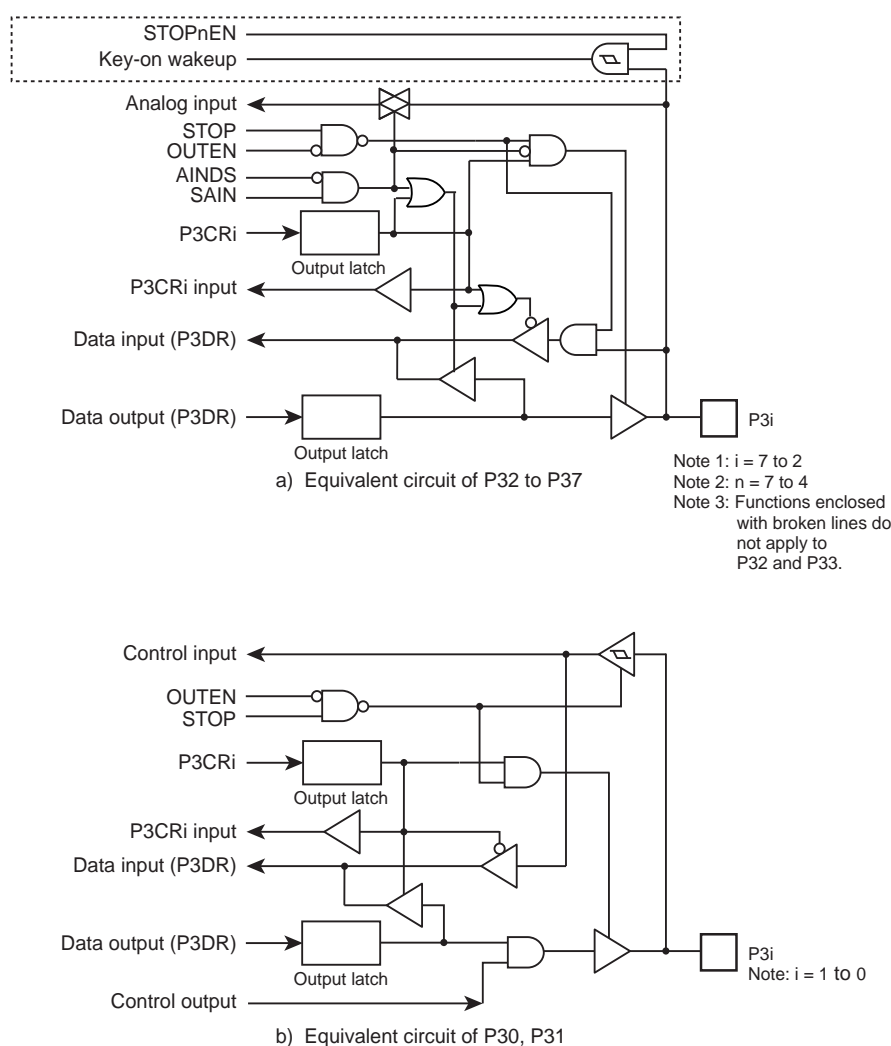
Figure 5-5 P3 Port
