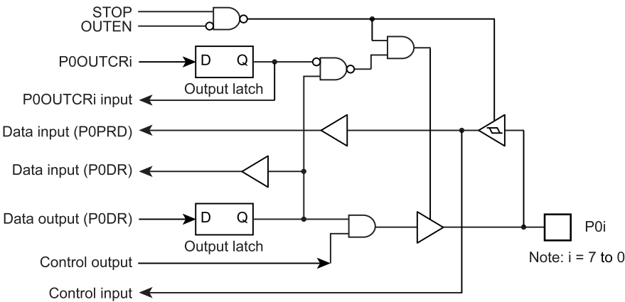
Figure 5-2 P0 Port
