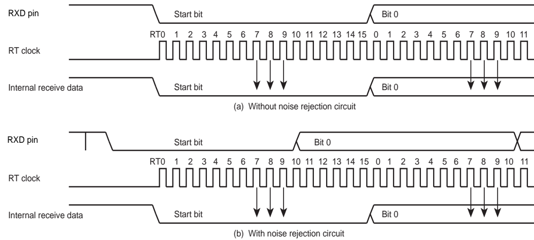
Figure 10-4 Data Sampling Method
