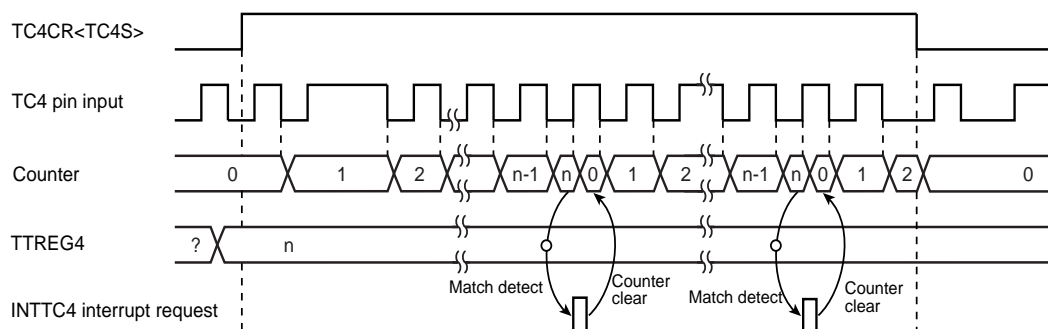
Figure 9-3 8-Bit Event Counter Mode Timing Chart (TC4)
