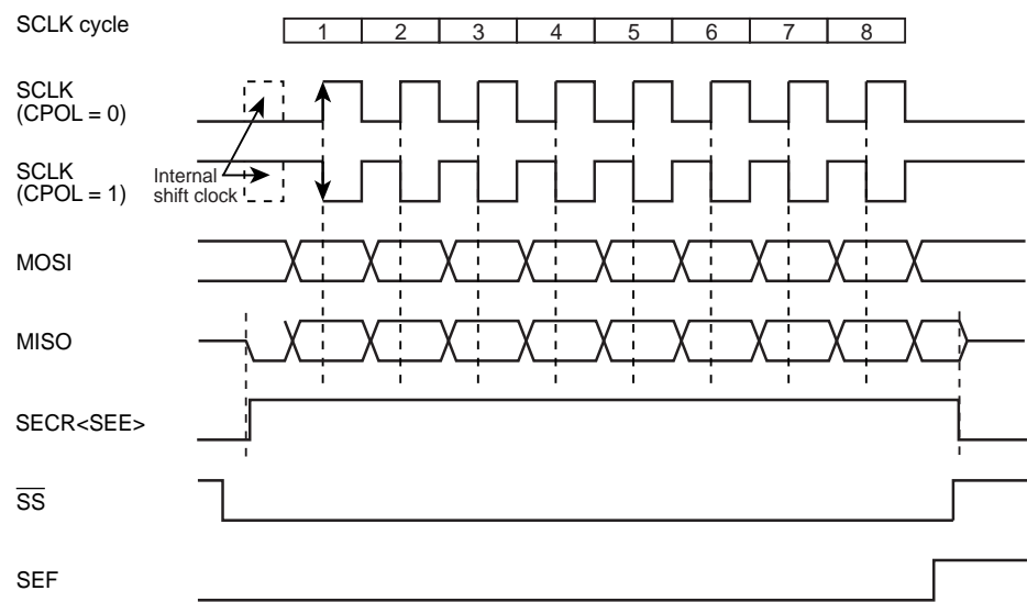
Figure 11-2 Transfer Format where CPHA = 0
