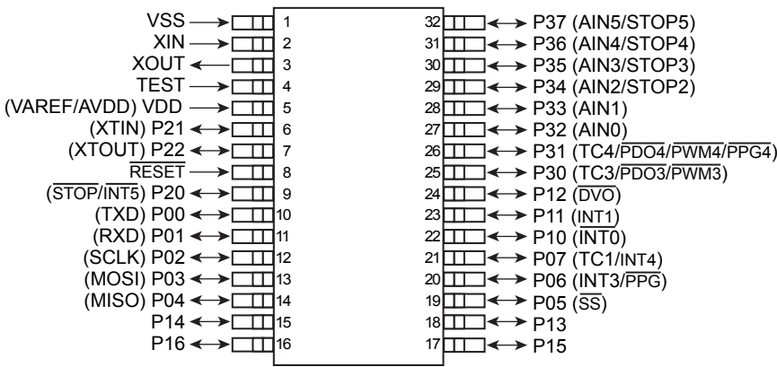
Figure 1-1 Pin Assignment
