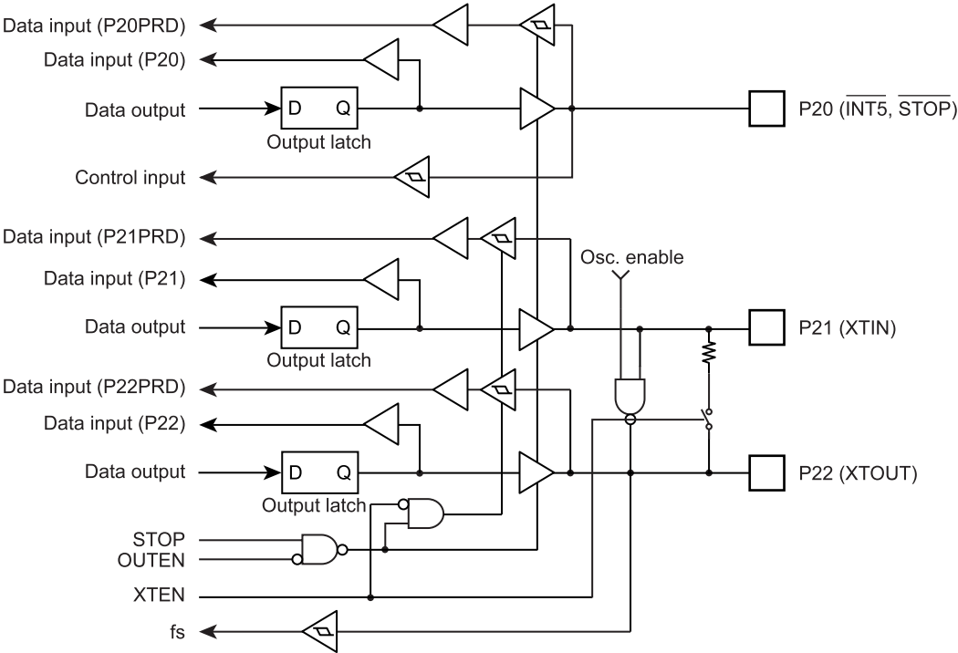
Figure 5-4 P2 Port
