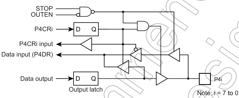
Figure 7-6 Port P4
