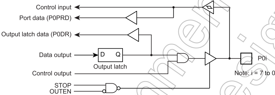
Figure 7-2 Port P0
