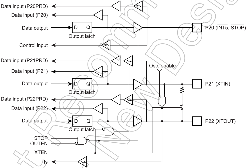
Figure 7-4 Port P2
