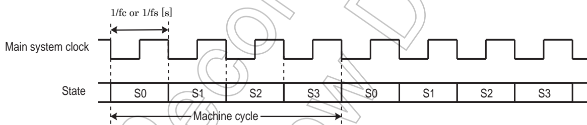
Figure 2-5 Machine Cycle
