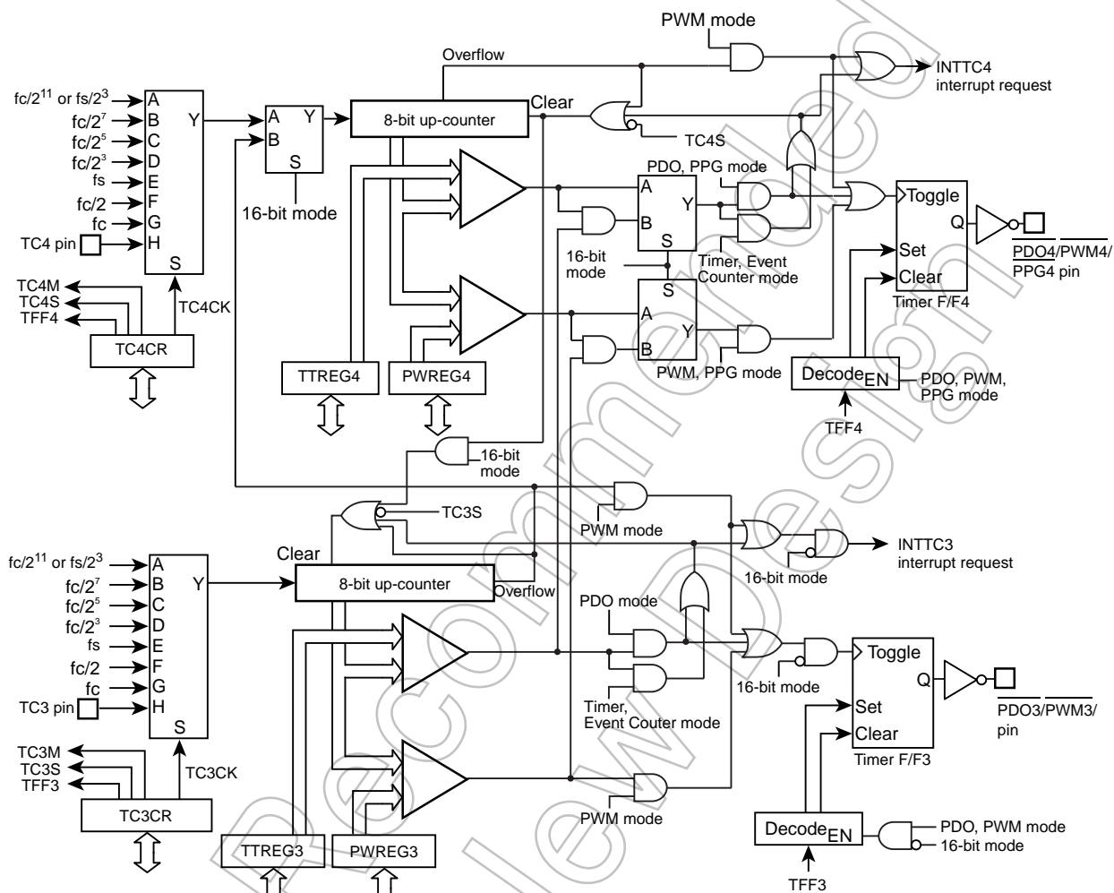
Figure 9-1 8-Bit TimerCounter 3, 4
