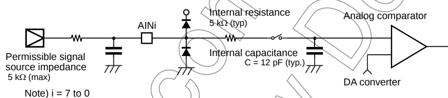
Figure 12-5 Analog Input Equivalent Circuit and Example of Input Pin Processing
