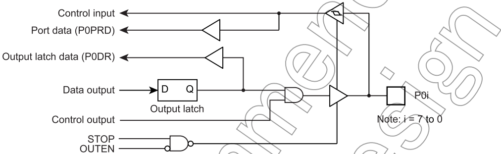
Figure 7-2 Port P0
