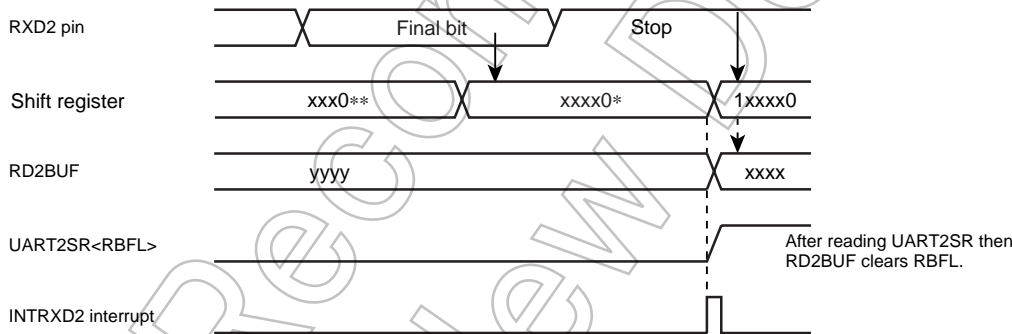
Figure 13-8 Generation of Receive Data Buffer Full
