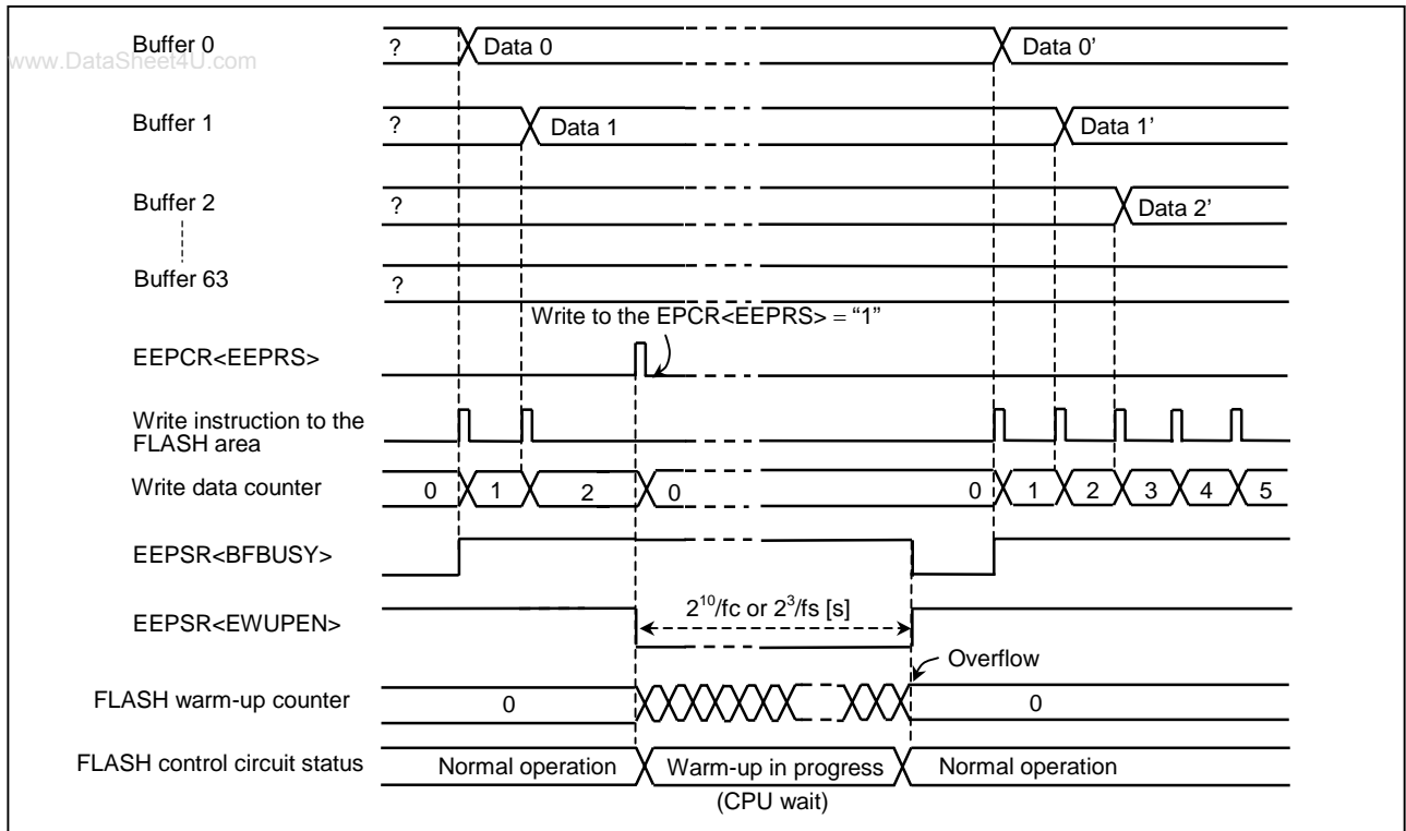
Figure 1.2.4 Write Data Counter Initialization and Write Forcible Stop
